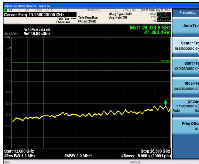
Band71-15MHz-QPSK-133397-1RB#0-Range1:0.009~0.15MHz
