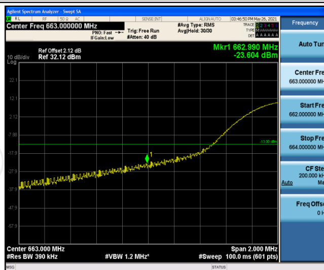
Band71-20MHz-16QAM-133222-1RB#99
