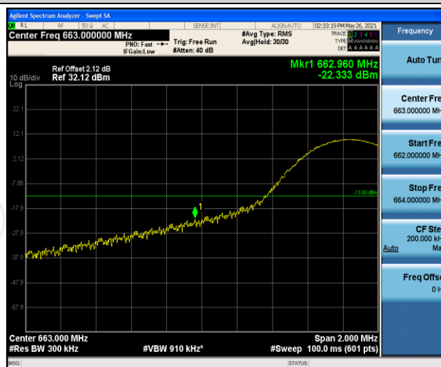
Band71-15MHz-QPSK-133197-1RB#74
