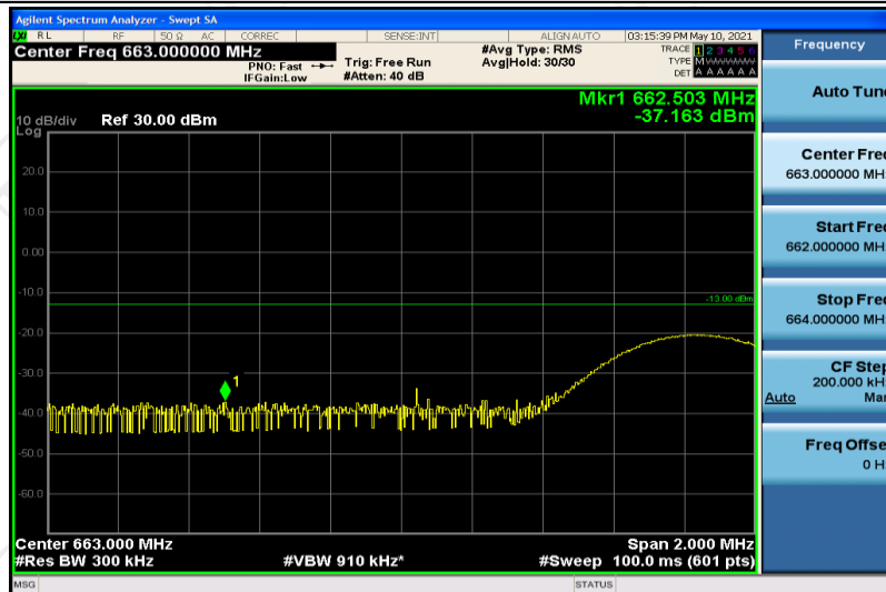
Band71-15MHz-QPSK-133197-1RB#0
