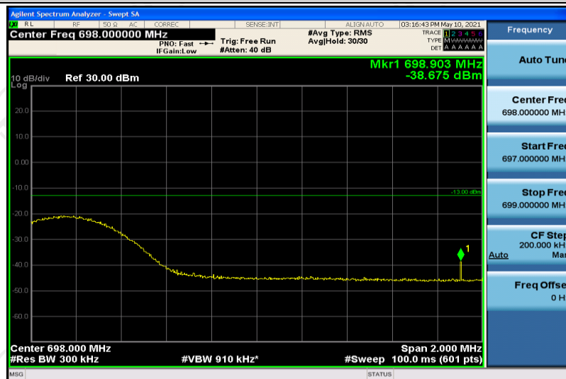
Band71-15MHz-16QAM-133397-1RB#74
