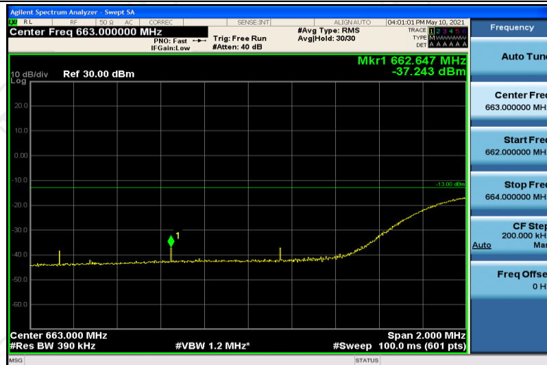
Band71-20MHz-16QAM-133222-1RB#0
