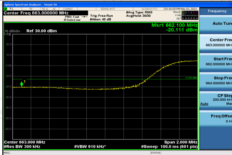
Band71-15MHz-QPSK-133397-1RB#0
