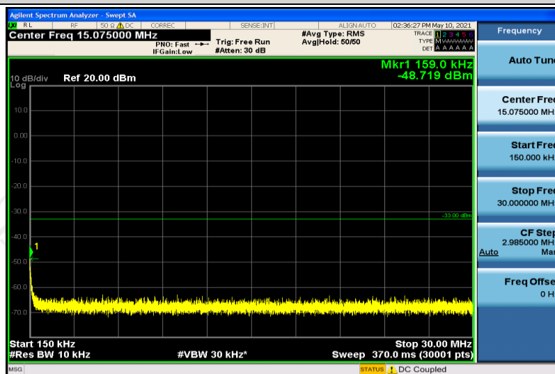
Band71-5MHz-QPSK-133297-1RB#0-Range3:30~1000MHz
