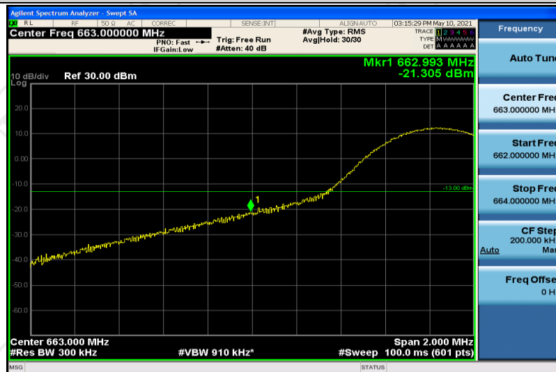
Band71-15MHz-16QAM-133197-1RB#74
