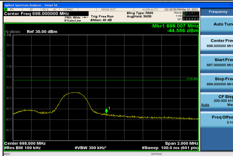
Band71-5MHz-QPSK-133447-1RB#24
