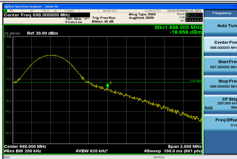
Band71-10MHz-16QAM-133422-50RB#0
