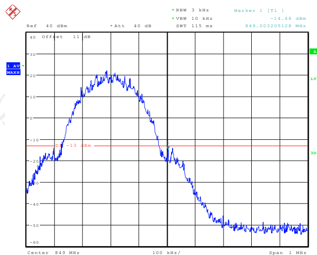
Higher Band Edge Plot on Channel 251
