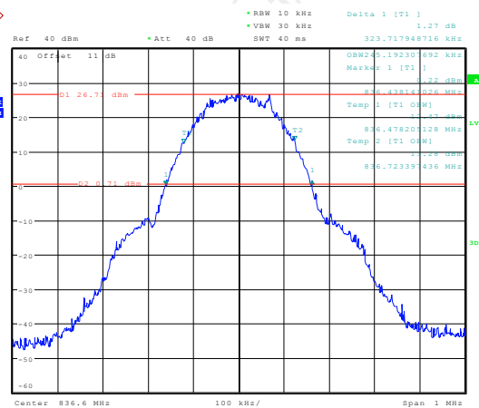
26dB&99% Occupied Bandwidth Plot on Channel 190
