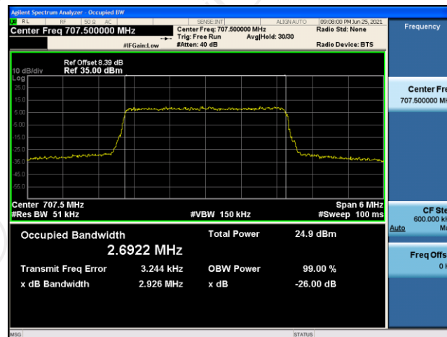
Band12-3MHz-16QAM-23165-15RB#0
