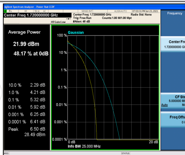
Band66-20MHz-QPSK-132322-1RB#0
