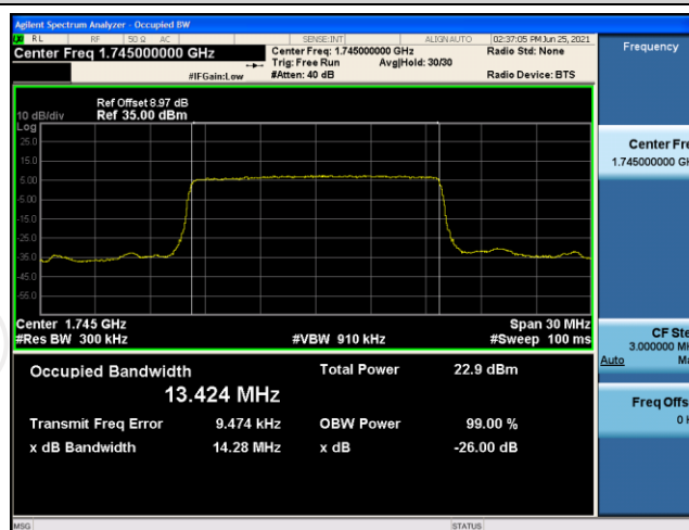
Band66-15MHz-16QAM-132597-75RB#0
