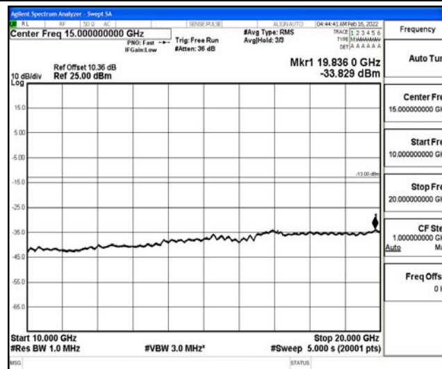
Band66-10MHz-QPSK-132322-1RB#0-Range1:0.009~0.15MHz
