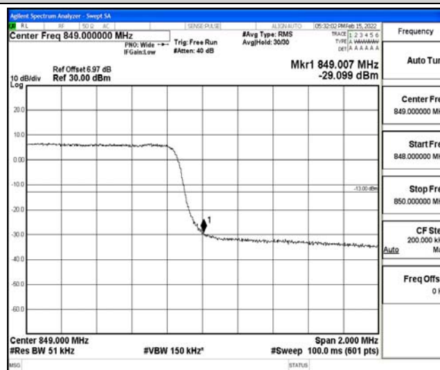
Band26-3MHz-16QAM-26805-15RB#0
