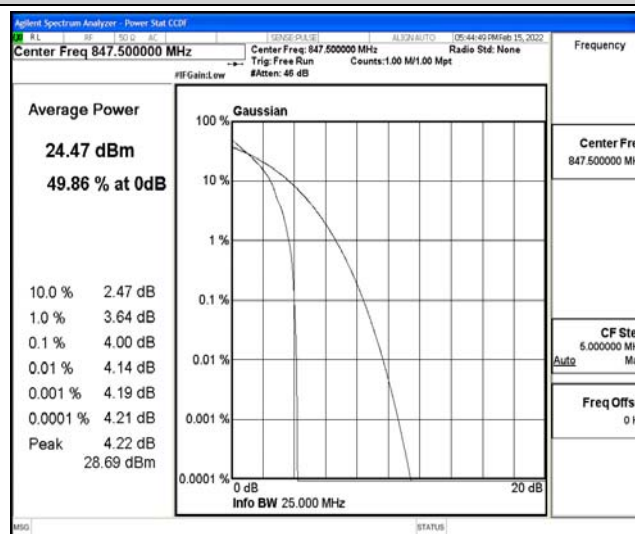
Band26-3MHz-QPSK-27025-15RB#0
