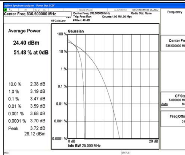
Band26-5MHz-QPSK-26915-25RB#0
