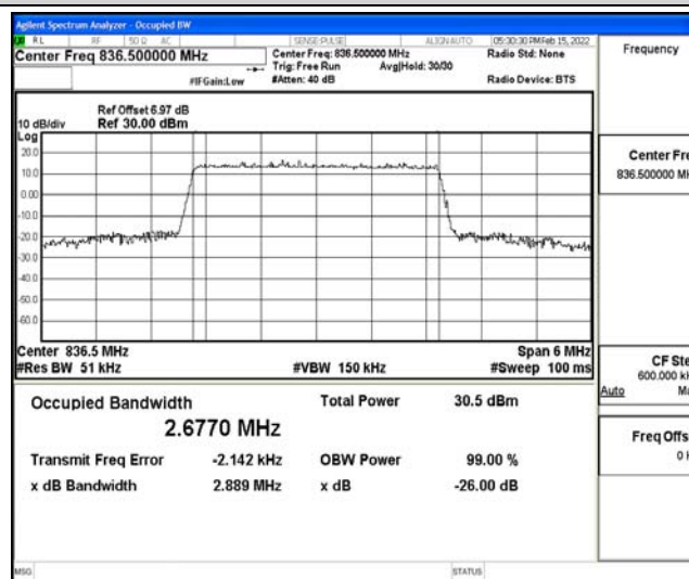
Band26-3MHz-16QAM-27025-15RB#0
