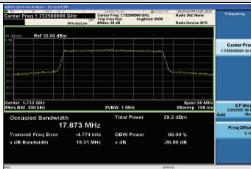
Band4-20MHz-16QAM-20175-100RB#0-17.873
