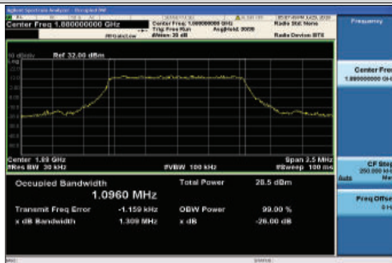
Band2-1.4MHz-QPSK-18900-6RB#0-1.0960
