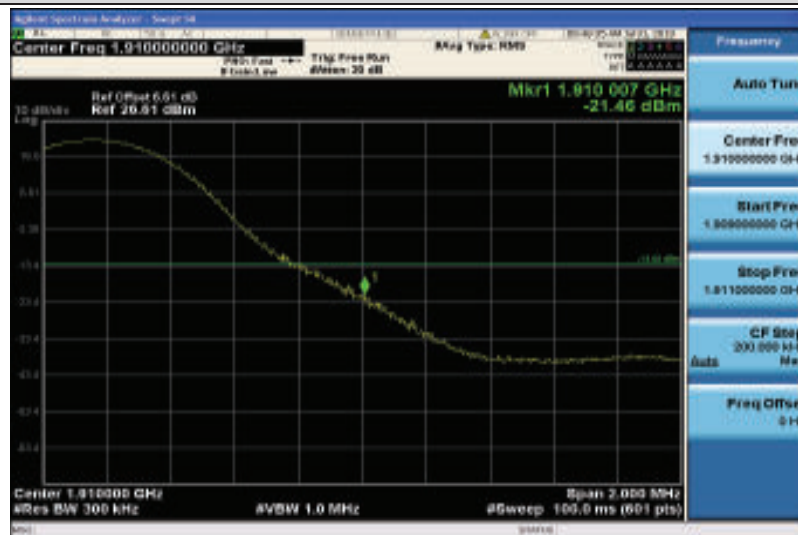
Band2-15MHz-QPSK-19125-1RB#74
