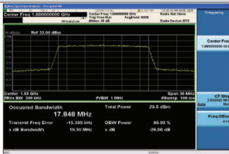
Band2-20MHz-QPSK-18900-100RB#0-17.848
