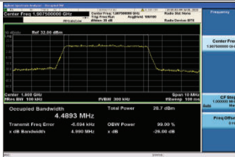
Band2-5MHz-16QAM-19175-25RB#0-4.4893
