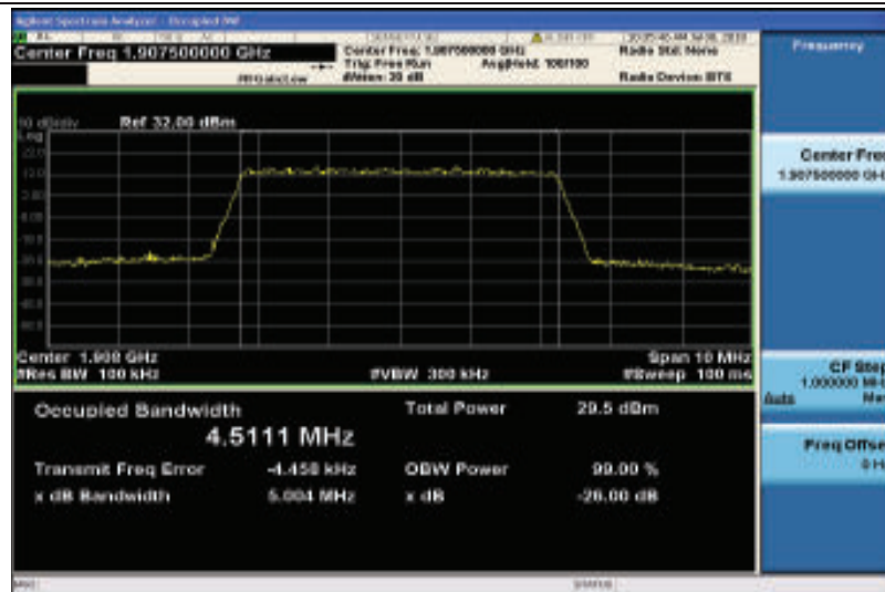
Band2-5MHz-QPSK-19175-25RB#0-4.5111
