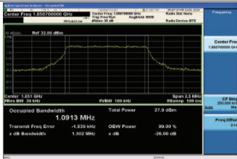
Band2-1.4MHz-16QAM-18607-6RB#0-1.0913
