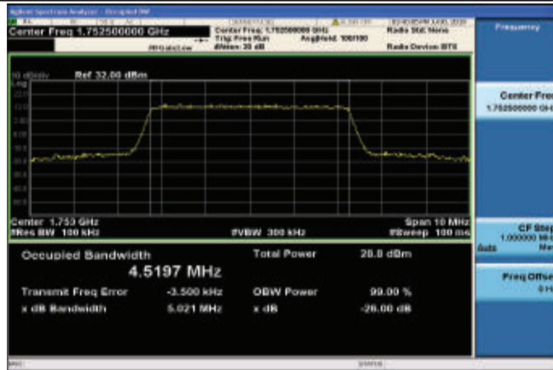
Band4-5MHz-16QAM-20375-25RB#0-4.5197
