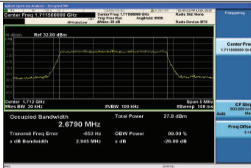
Band4-3MHz-16QAM-19965-15RB#0-2.6790
