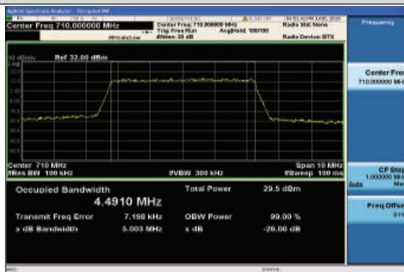
Band17-5MHz-QPSK-23790-25RB#0-4.4910
