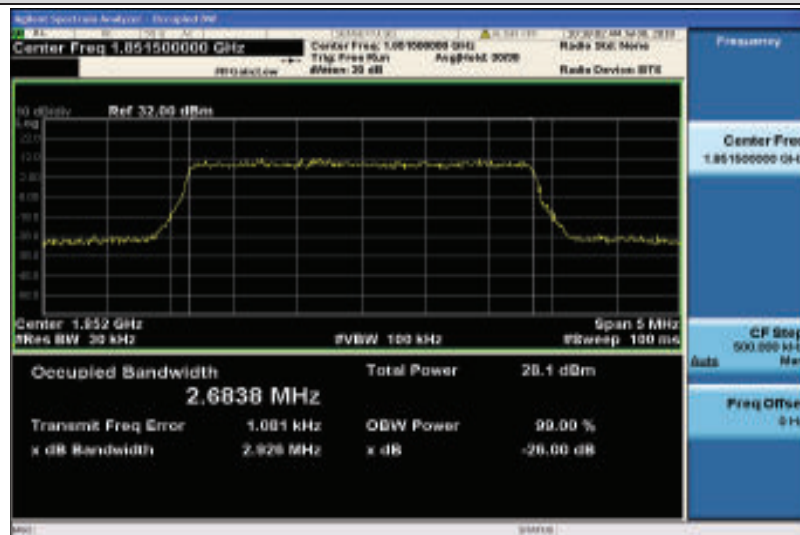
Band2-3MHz-16QAM-18615-15RB#0-2.6838
