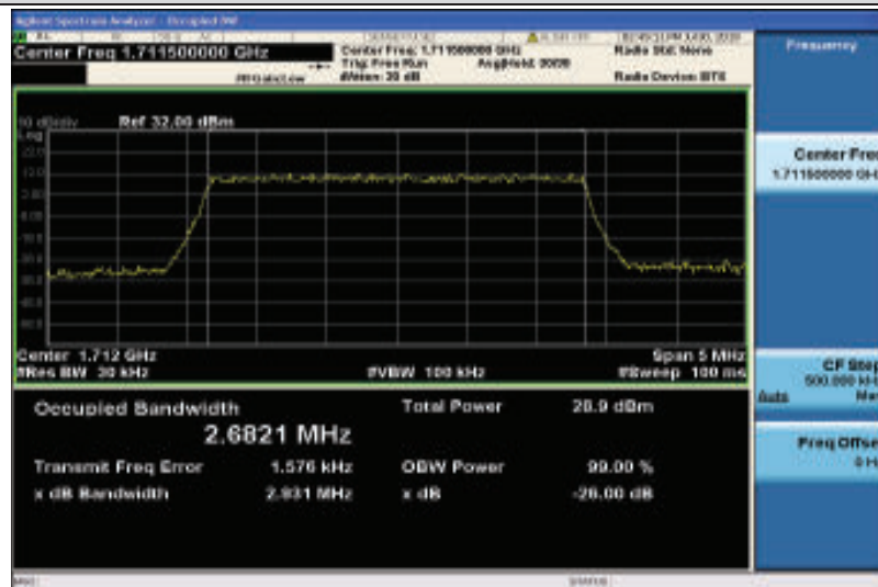
Band4-3MHz-QPSK-19965-15RB#0-2.6821
