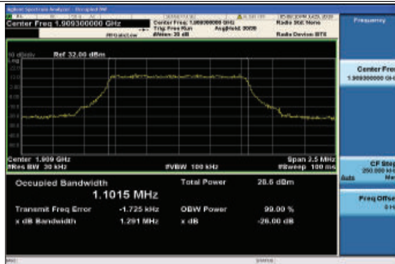
Band2-1.4MHz-QPSK-19193-6RB#0-1.1015
