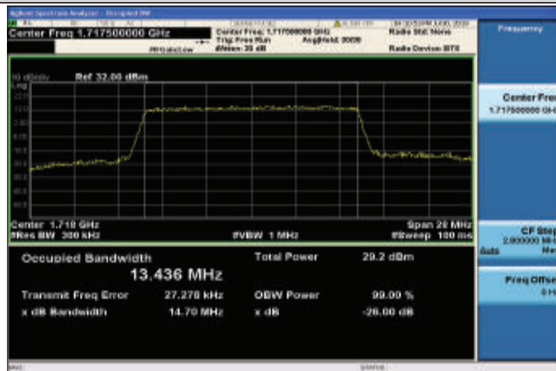
Band4-15MHz-16QAM-20025-75RB#0-13.436
