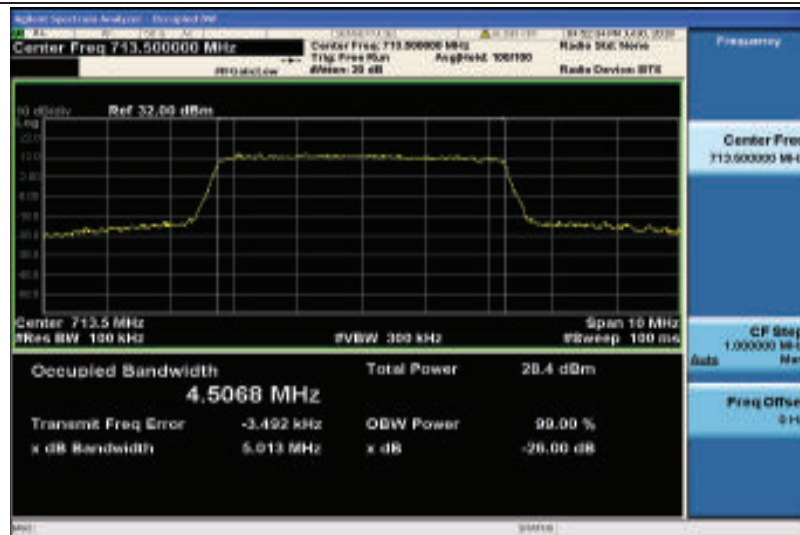
Band17-5MHz-16QAM-23825-25RB#0-4.5068
