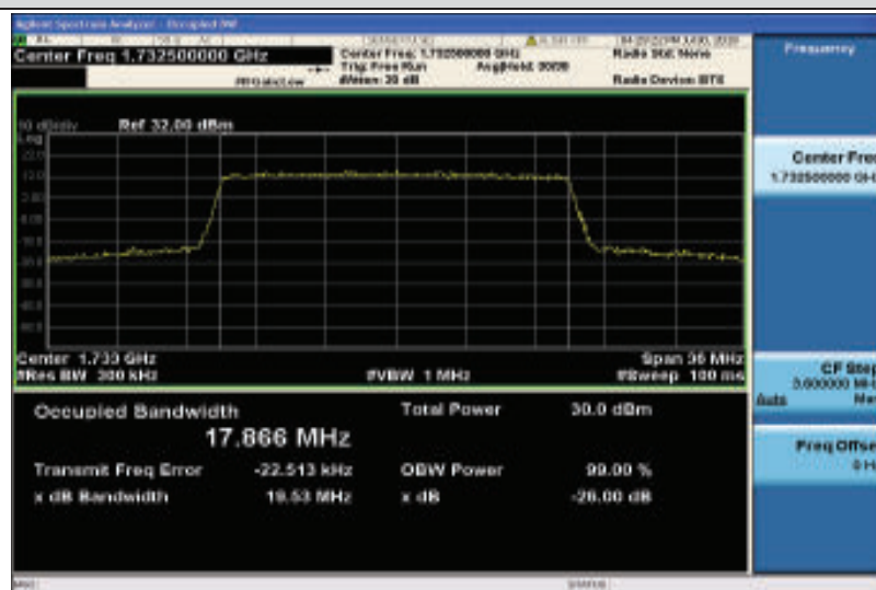
Band4-20MHz-QPSK-20175-100RB#0-17.866
