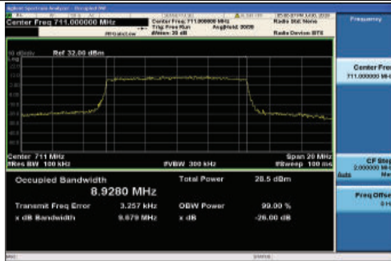
Band17-10MHz-16QAM-23800-50RB#0-8.9280
