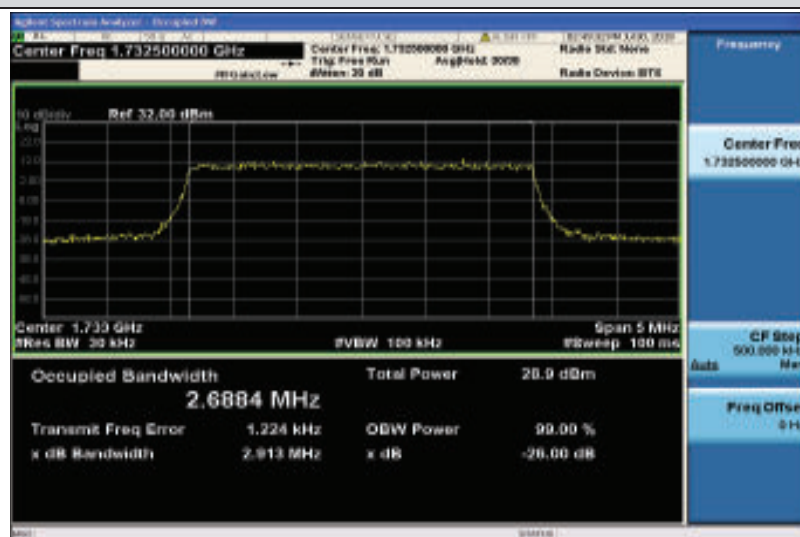
Band4-3MHz-QPSK-20175-15RB#0-2.6884
