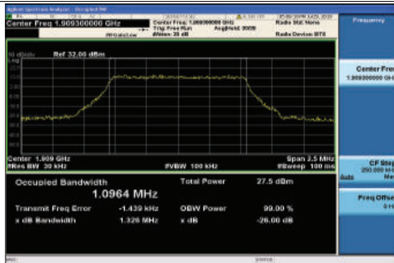
Band2-1.4MHz-16QAM-19193-6RB#0-1.0964
