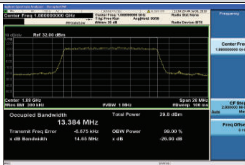
Band2-15MHz-QPSK-18900-75RB#0-13.384
