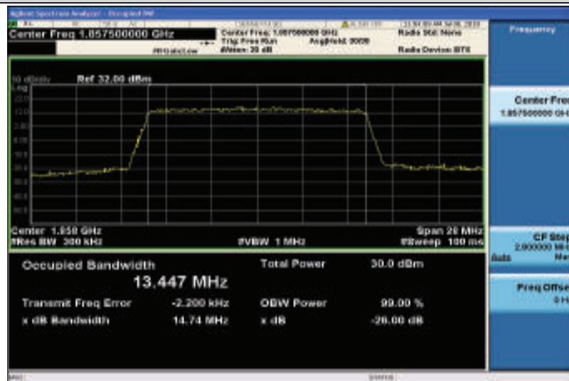
Band2-15MHz-QPSK-18675-75RB#0-13.447
