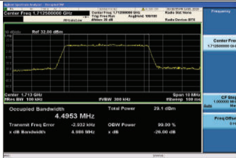
Band4-5MHz-16QAM-19975-25RB#0-4.4953
