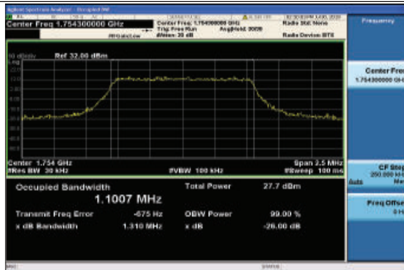
Band4-1.4MHz-16QAM-20393-6RB#0-1.1007
