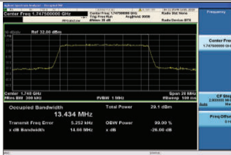
Band4-15MHz-16QAM-20325-75RB#0-13.434
