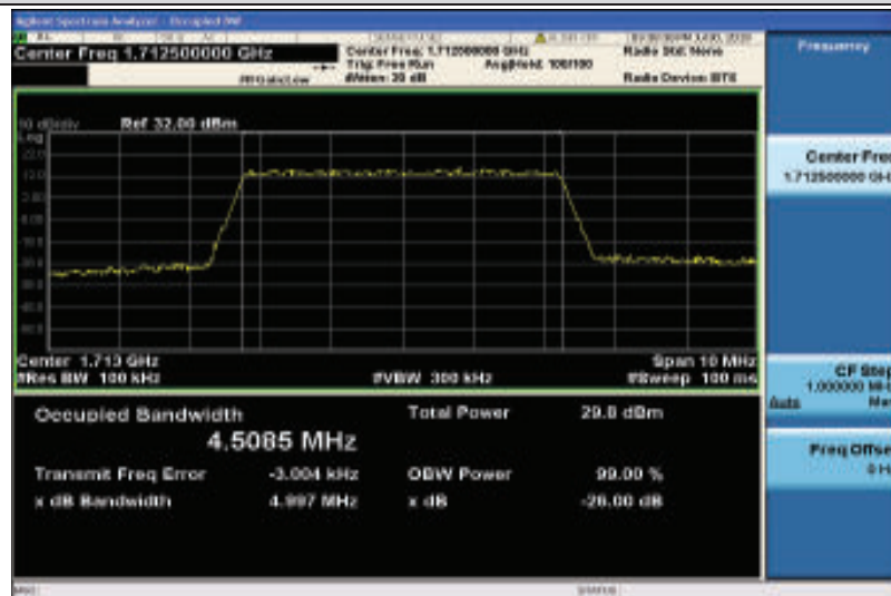
Band4-5MHz-QPSK-19975-25RB#0-4.5085
