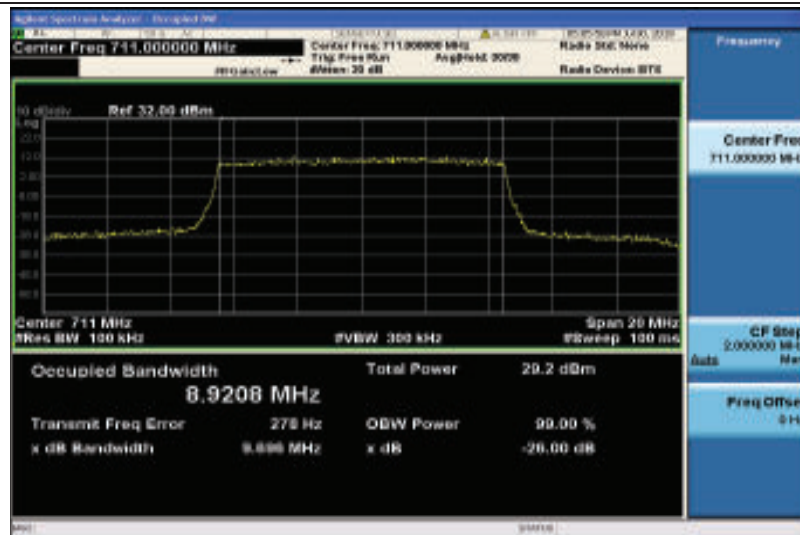
Band17-10MHz-QPSK-23800-50RB#0-8.9208
