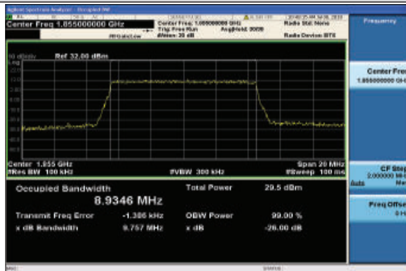
Band2-10MHz-QPSK-18650-50RB#0-8.9346
