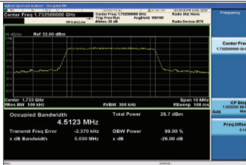
Band4-5MHz-16QAM-20175-25RB#0-4.5123
