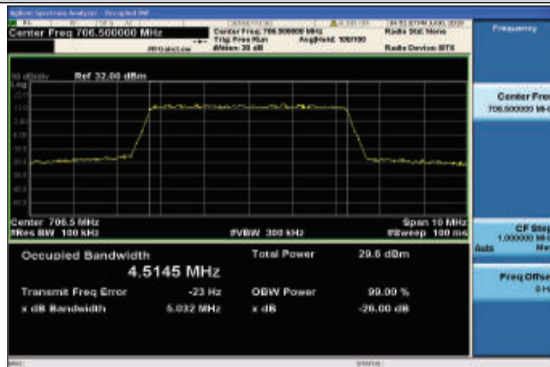
Band17-5MHz-QPSK-23755-25RB#0-4.5145
