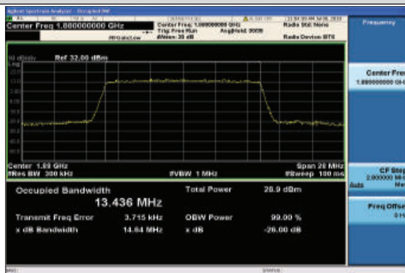
Band2-15MHz-16QAM-18900-75RB#0-13.436
