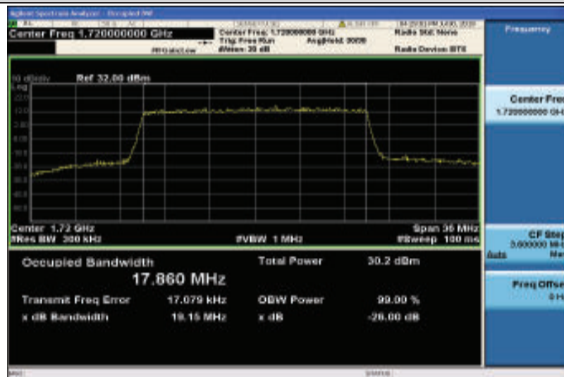
Band4-20MHz-QPSK-20050-100RB#0-17.860
