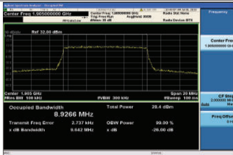
Band2-10MHz-16QAM-19150-50RB#0-8.9266
