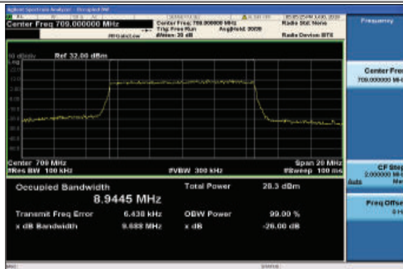
Band17-10MHz-16QAM-23780-50RB#0-8.9445
