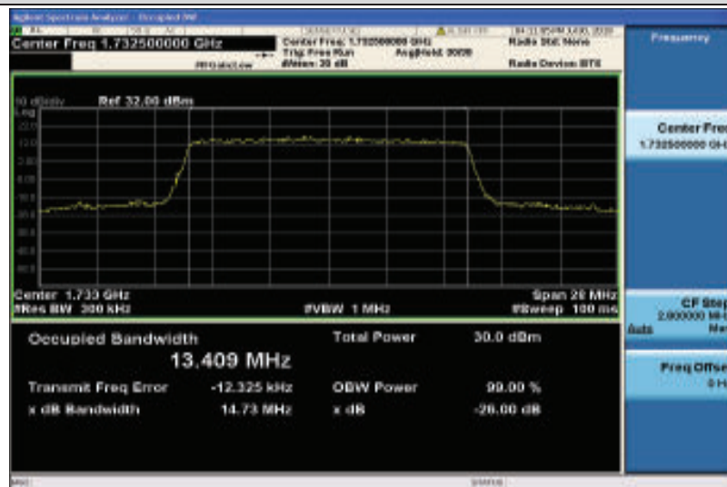
Band4-15MHz-QPSK-20175-75RB#0-13.409
