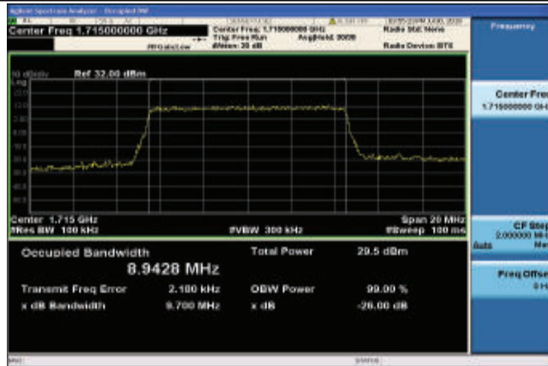
Band4-10MHz-QPSK-20000-50RB#0-8.9428
