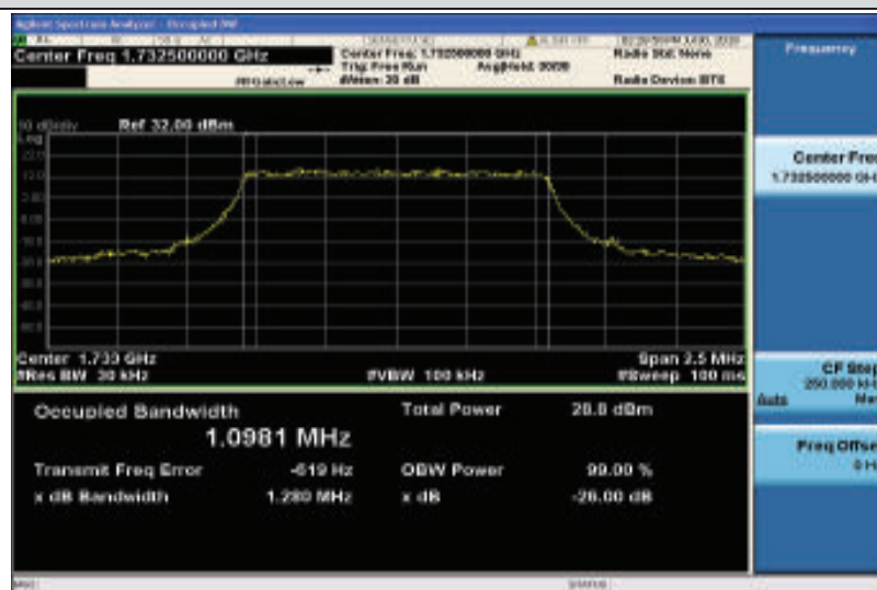
Band4-1.4MHz-QPSK-20175-6RB#0-1.0981
