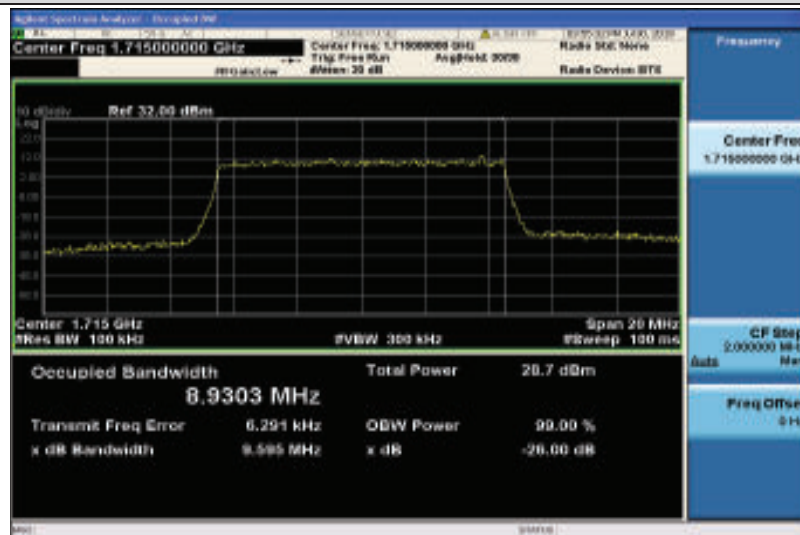
Band4-10MHz-16QAM-20000-50RB#0-8.9303
