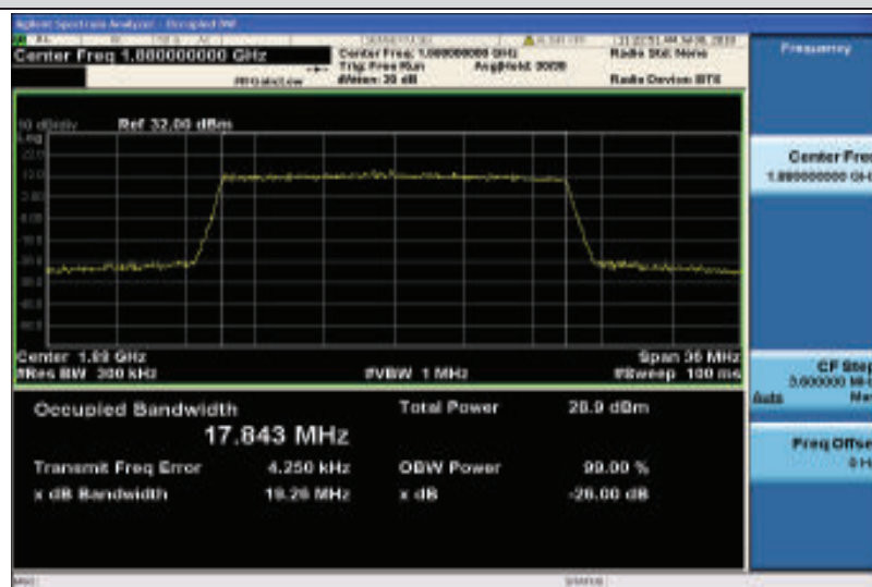
Band2-20MHz-16QAM-18900-100RB#0-17.843
