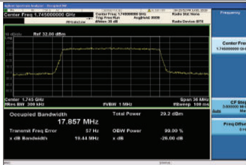
Band4-20MHz-16QAM-20300-100RB#0-17.857
