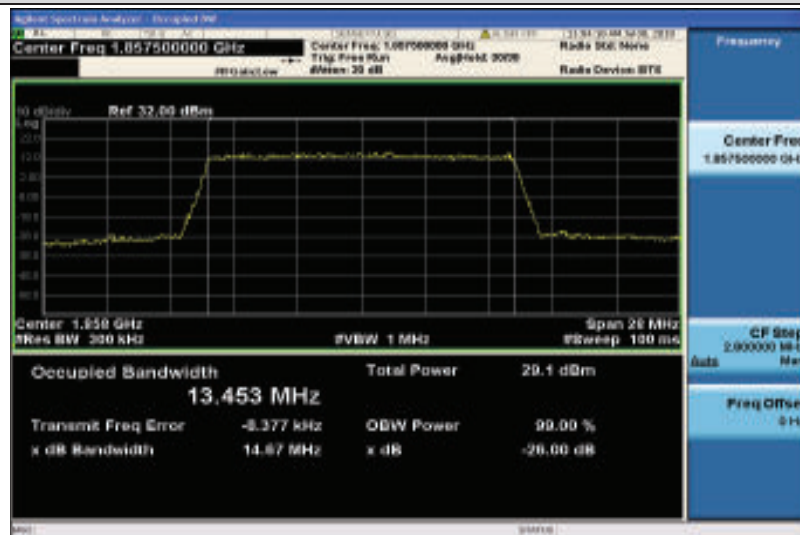
Band2-15MHz-16QAM-18675-75RB#0-13.453
