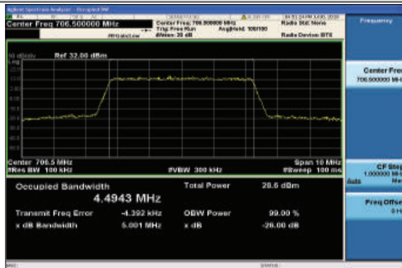
Band17-5MHz-16QAM-23755-25RB#0-4.4943
