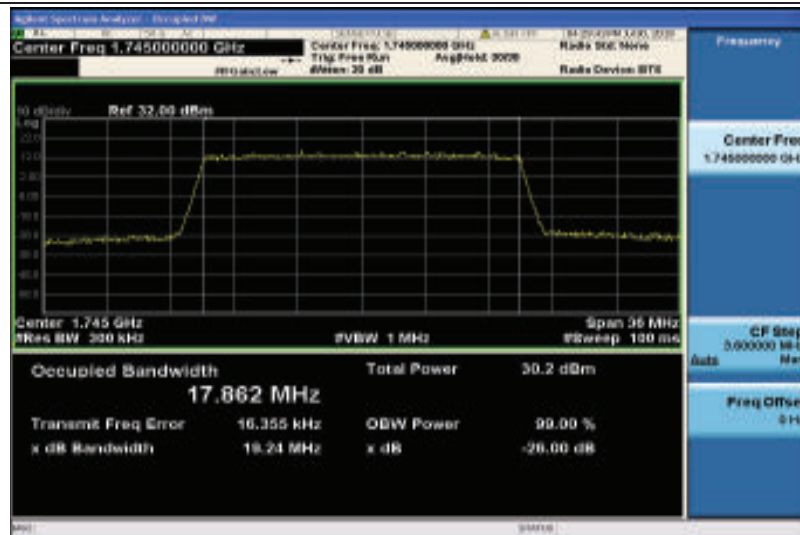
Band4-20MHz-QPSK-20300-100RB#0-17.862
