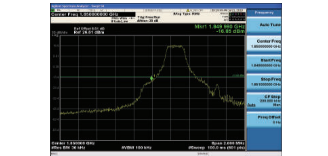
Band2-1.4MHz-QPSK-18607-1RB#0
