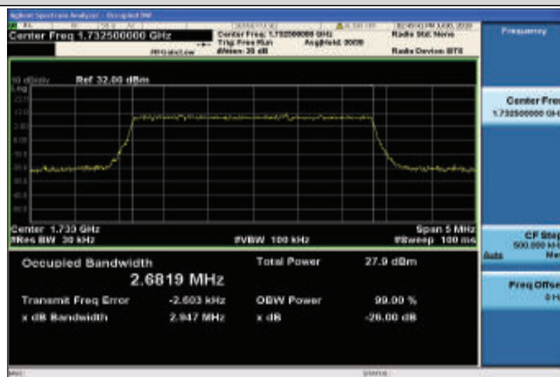
Band4-3MHz-16QAM-20175-15RB#0-2.6819
