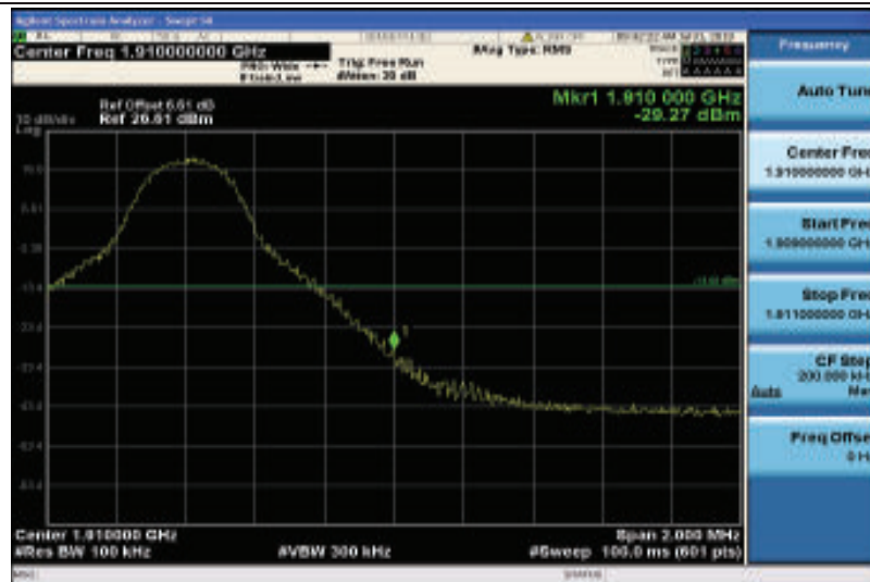
Band2-10MHz-16QAM-19150-1RB#49
