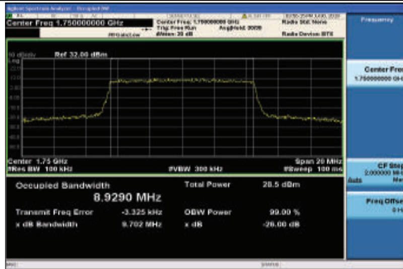
Band4-10MHz-16QAM-20350-50RB#0-8.9290
