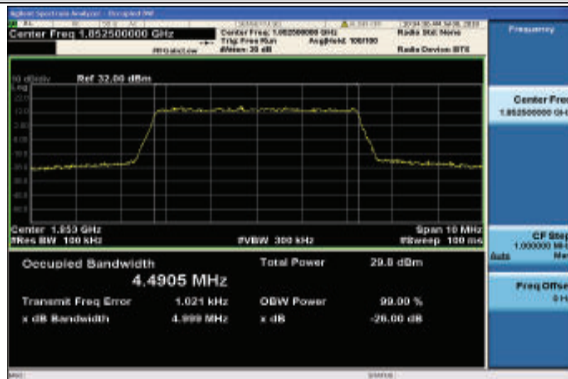
Band2-5MHz-QPSK-18625-25RB#0-4.4905
