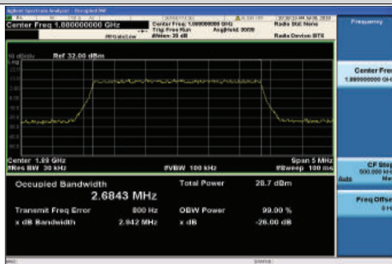
Band2-3MHz-QPSK-18900-15RB#0-2.6843
