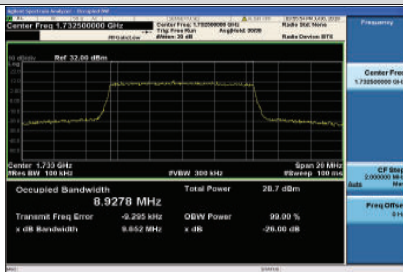
Band4-10MHz-16QAM-20175-50RB#0-8.9278
