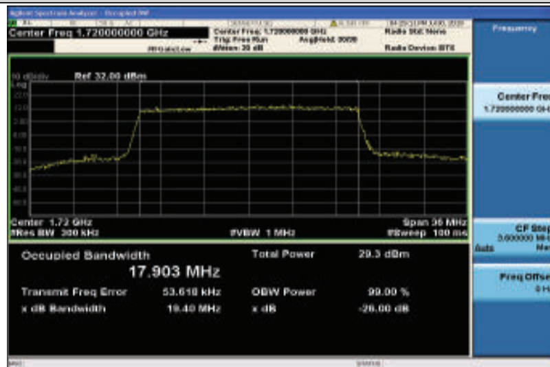
Band4-20MHz-16QAM-20050-100RB#0-17.903
