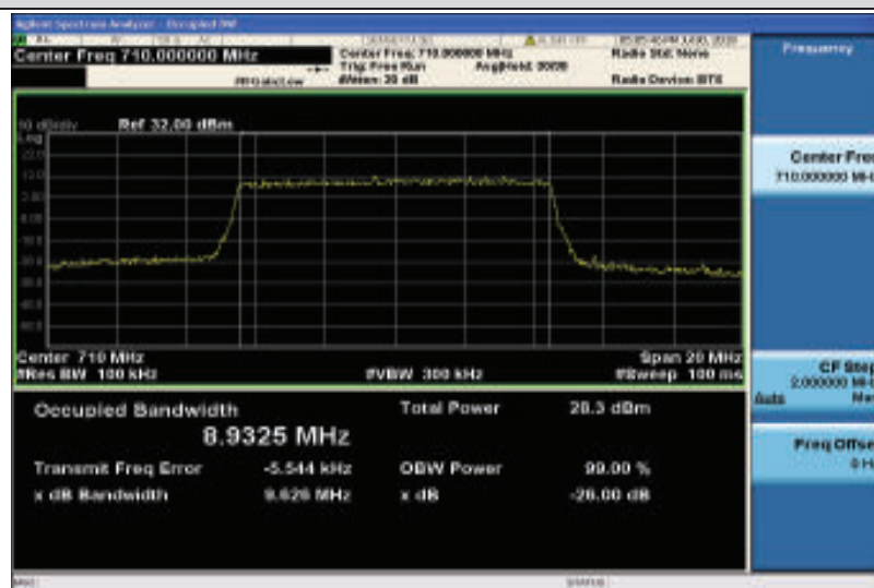
Band17-10MHz-16QAM-23790-50RB#0-8.9325
