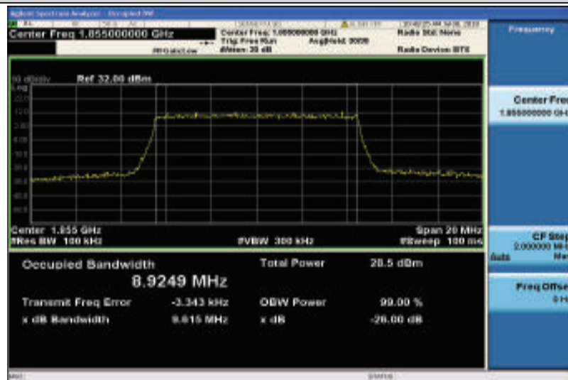
Band2-10MHz-16QAM-18650-50RB#0-8.9249
