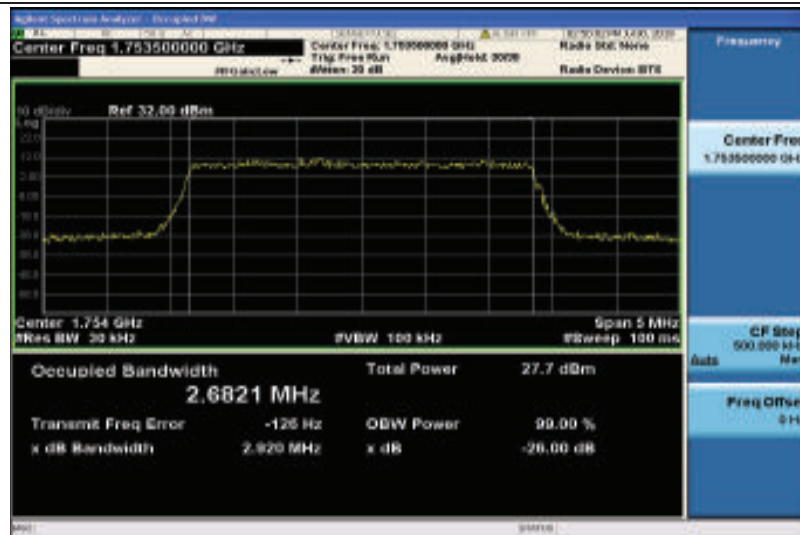
Band4-3MHz-16QAM-20385-15RB#0-2.6821
