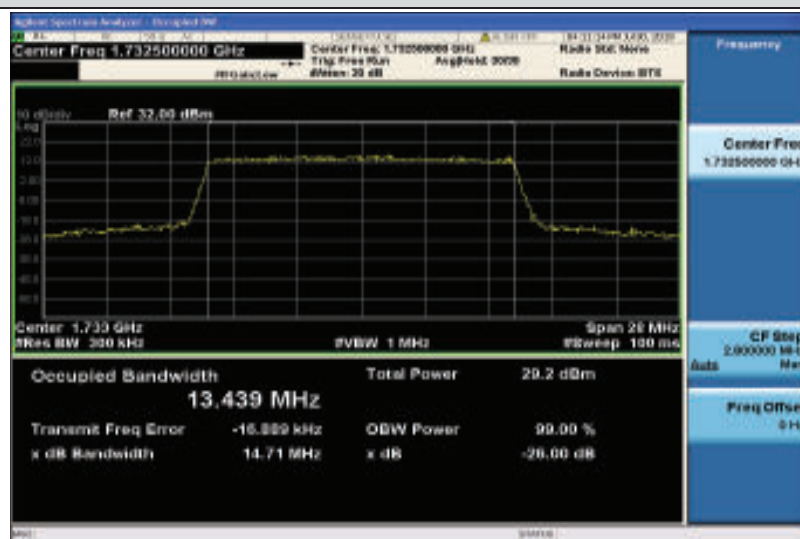
Band4-15MHz-16QAM-20175-75RB#0-13.439
