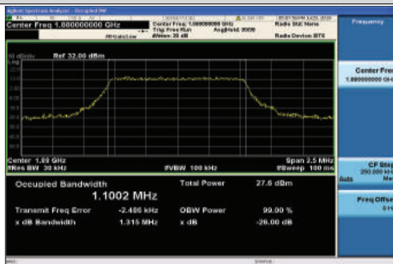
Band2-1.4MHz-16QAM-18900-6RB#0-1.1002
