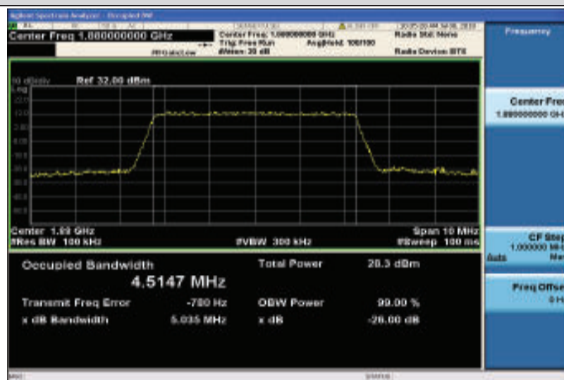
Band2-5MHz-16QAM-18900-25RB#0-4.5147
