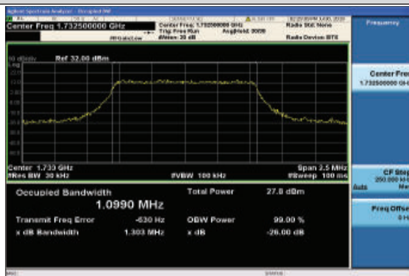
Band4-1.4MHz-16QAM-20175-6RB#0-1.0990
