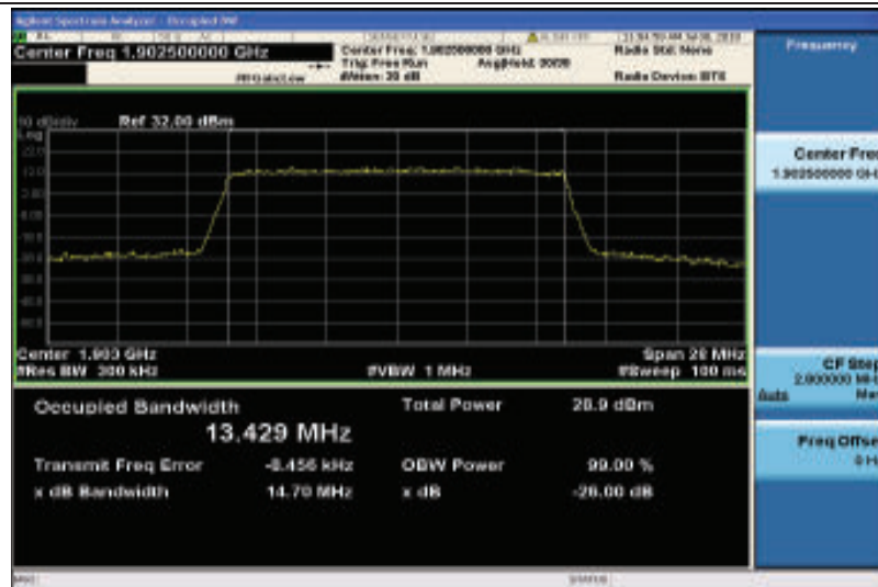
Band2-15MHz-16QAM-19125-75RB#0-13.429
