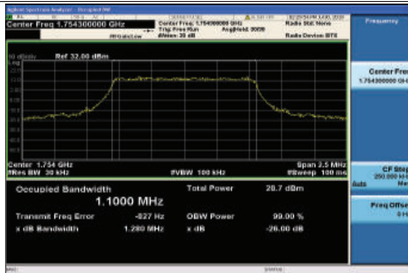
Band4-1.4MHz-QPSK-20393-6RB#0-1.1000
