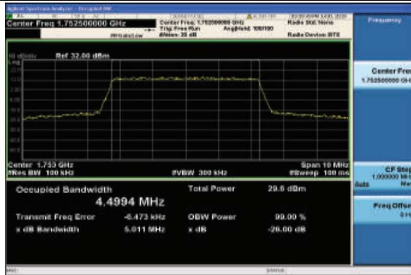
Band4-5MHz-QPSK-20375-25RB#0-4.4994
