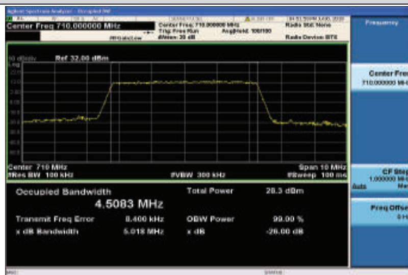
Band17-5MHz-16QAM-23790-25RB#0-4.5083
