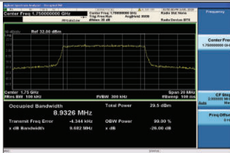
Band4-10MHz-QPSK-20350-50RB#0-8.9326
