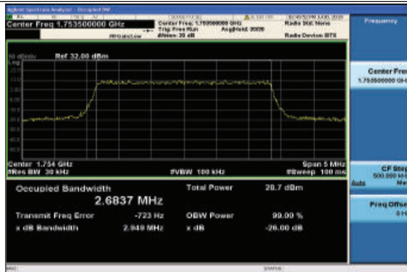
Band4-3MHz-QPSK-20385-15RB#0-2.6837
