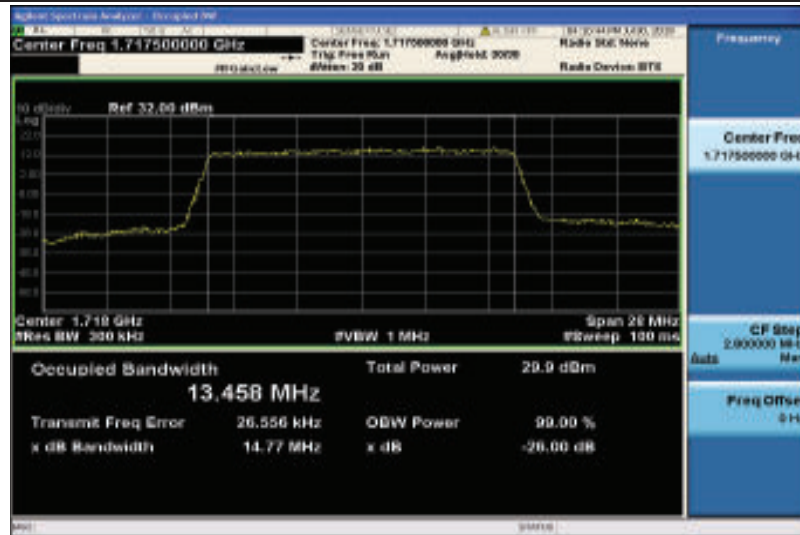
Band4-15MHz-QPSK-20025-75RB#0-13.458
