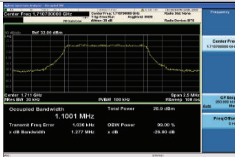
Band4-1.4MHz-QPSK-19957-6RB#0-1.1001
