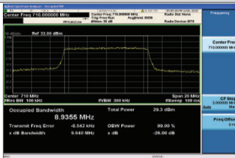
Band17-10MHz-QPSK-23790-50RB#0-8.9355
