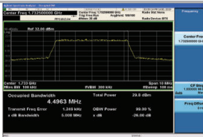
Band4-5MHz-QPSK-20175-25RB#0-4.4963
