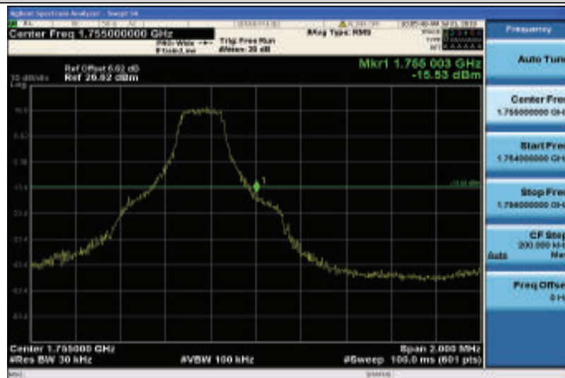
Band4-3MHz-QPSK-20385-1RB#14
