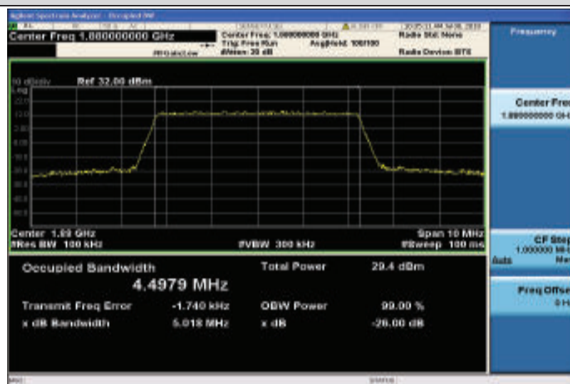
Band2-5MHz-QPSK-18900-25RB#0-4.4979
