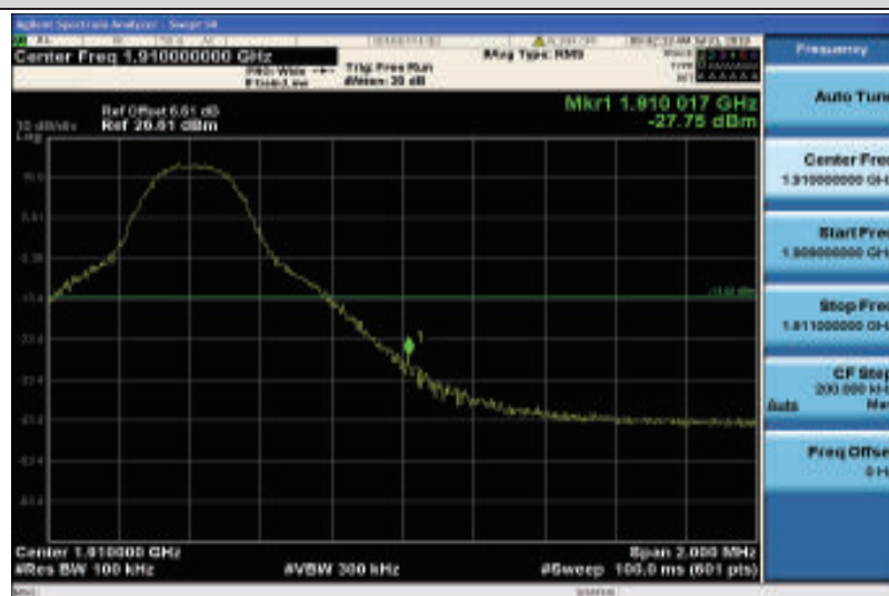
Band2-10MHz-QPSK-19150-1RB#49
