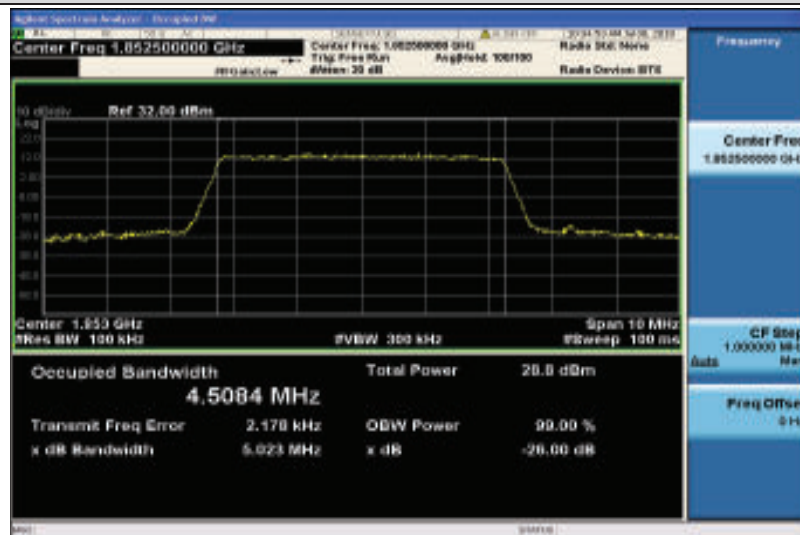
Band2-5MHz-16QAM-18625-25RB#0-4.5084
