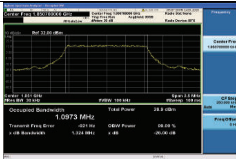
Band2-1.4MHz-QPSK-18607-6RB#0-1.0973
