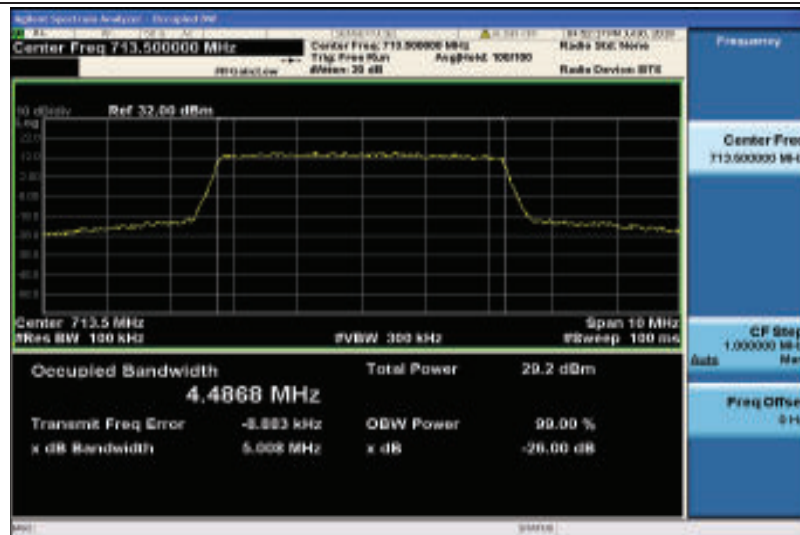
Band17-5MHz-QPSK-23825-25RB#0-4.4868
