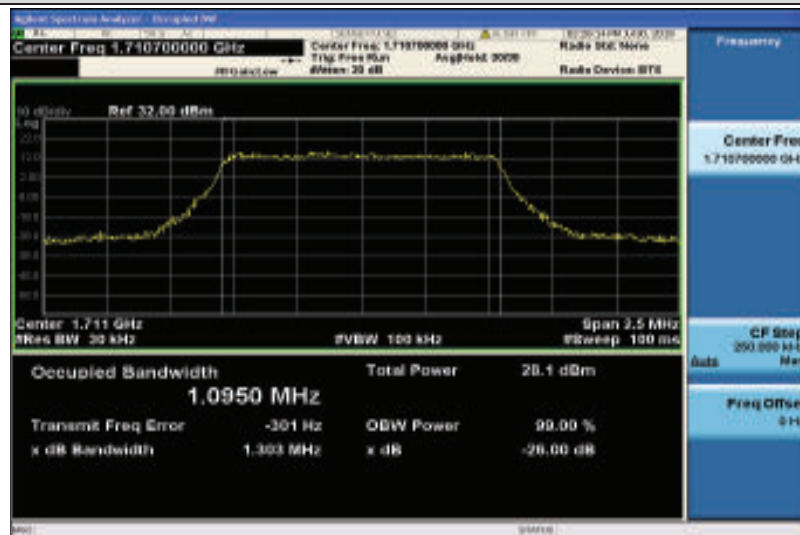
Band4-1.4MHz-16QAM-19957-6RB#0-1.0950
