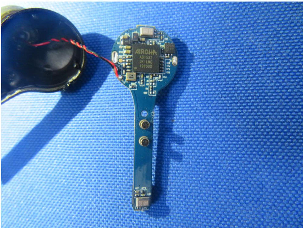
(4) EUT Photo (Left Headphone)
