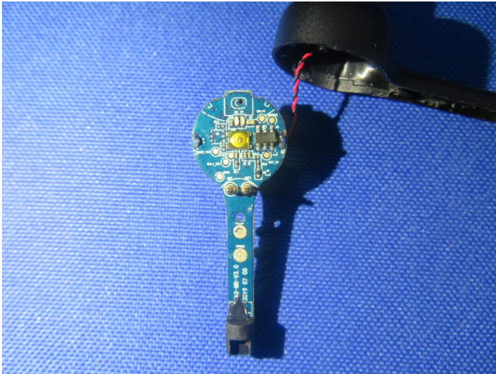
(3) EUT Photo (Left Headphone)
