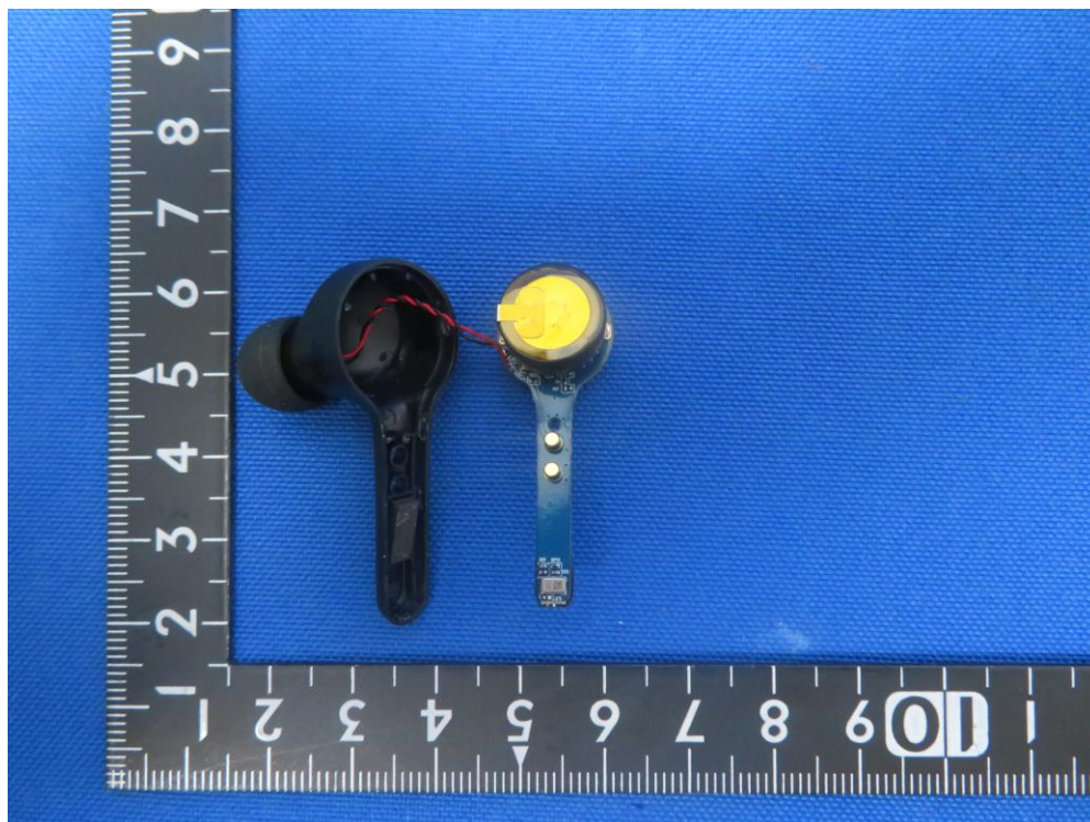
(2) EUT Photo (Left Headphone)
