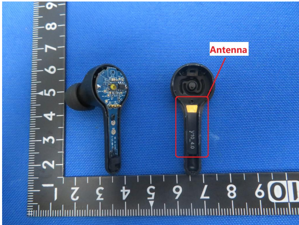
(1) EUT Photo (Left Headphone)
