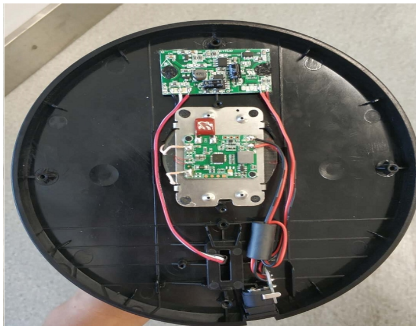
EUT – Cover off View-4 Without Indicator Light
