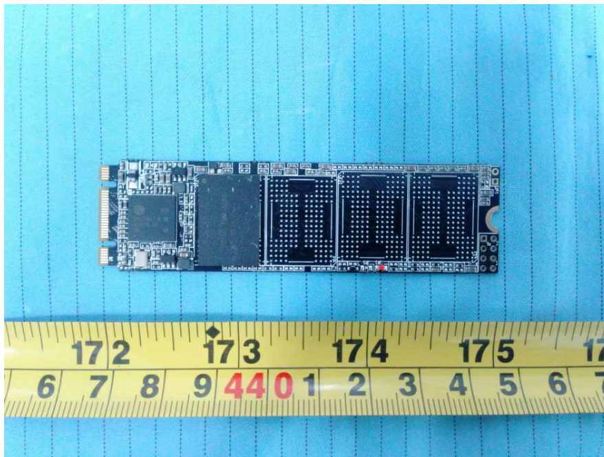
EUT –Small Board 1 Top Shielding off View
