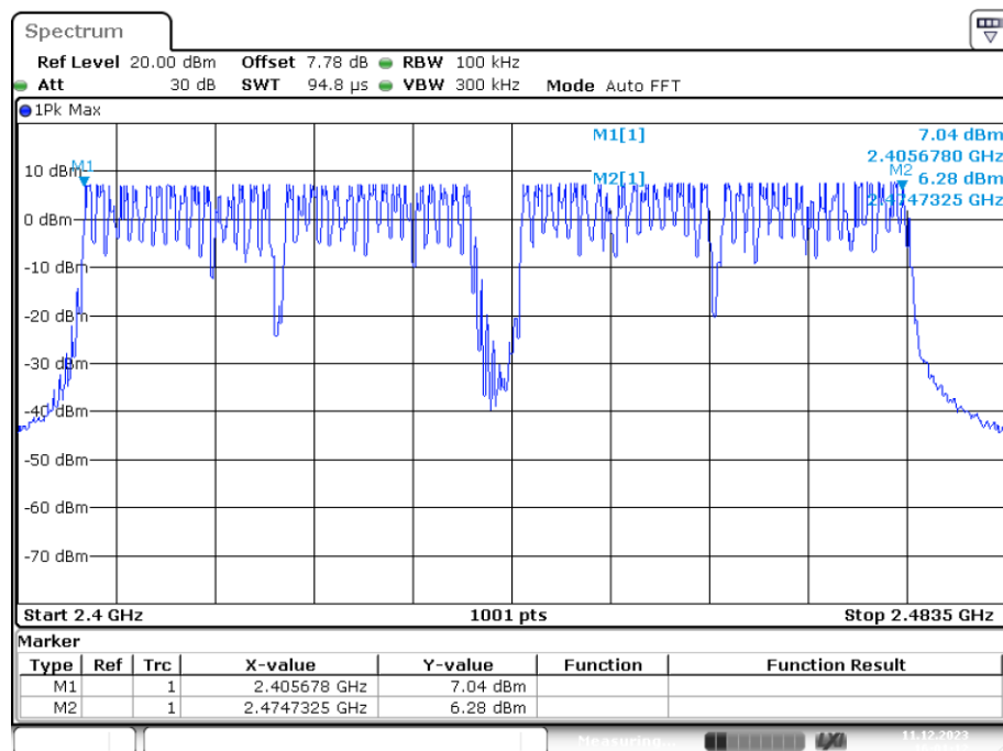
Hopping No. NVNT GFSK 2443MHz Ant1
