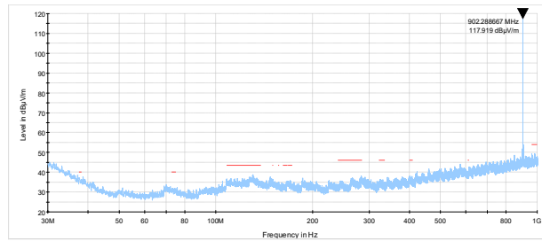
Figure 8.8-10: Radiated spurious emissions 30 – 1000 MHz, LoRa 125 kHz BW, Low channel 902.3 MHz
