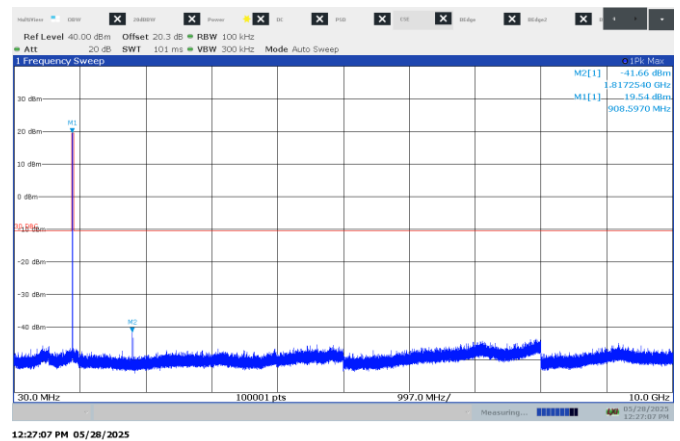
Figure 8.8-2: Conducted spurious emissions on mid channel, 125 kHz BW
