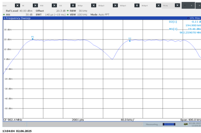
Figure 7.4-5: Carrier frequency separation
