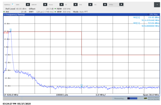
Figure 8.8-18: Conducted Band-edge on high channel, 500 kHz BW
