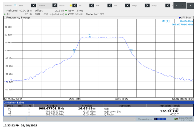
Figure 7.4-2: 20 dB bandwidth on mid channel – 125 kHz BW
