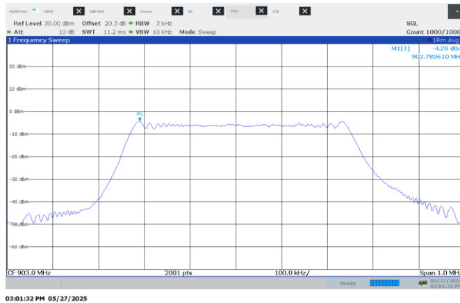
Figure 8.9-1: PSD on low channel, 500 kHz BW
