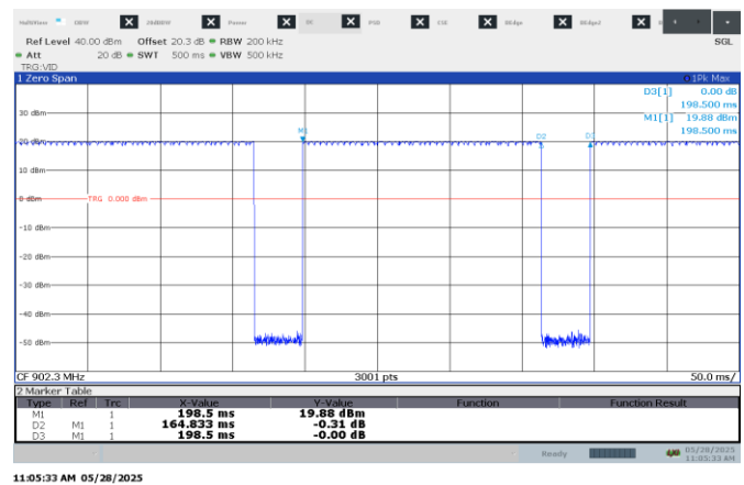
Figure 8.5-4: Duty cycle, 125 kHz BW
