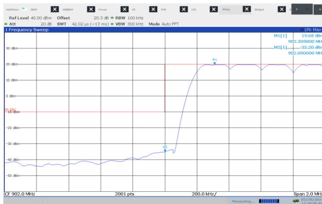
Figure 8.8-6: Conducted Band edge on low channel hopping, 125 kHz BW
