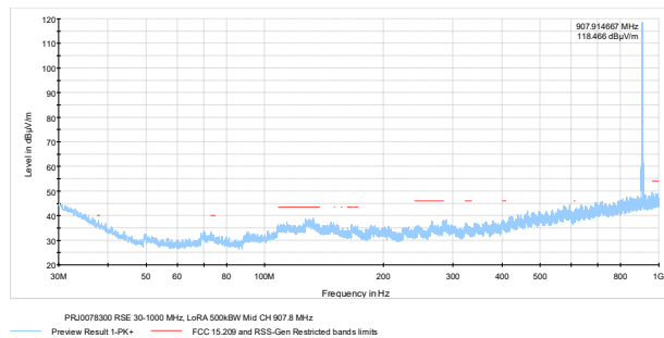
Figure 8.8-10: Radiated spurious emissions 30 – 1000 MHz, LoRa 500 kHz BW, Mid channel 907.8 MHz
