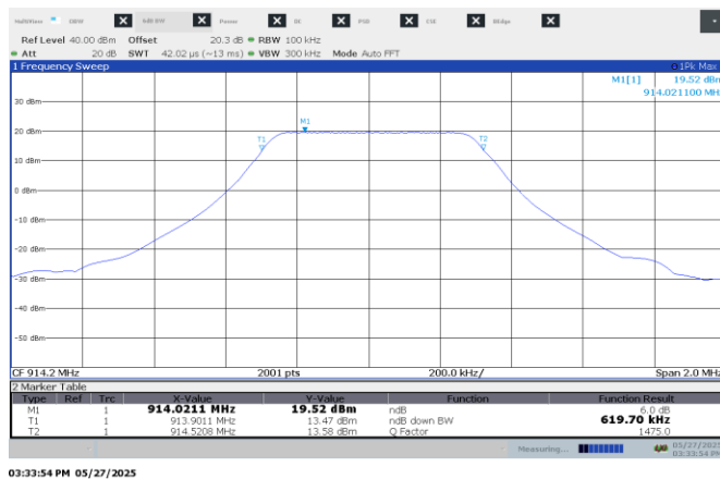
Figure 8.6-3: 6 dB bandwidth on high channel – 500 kHz BW
