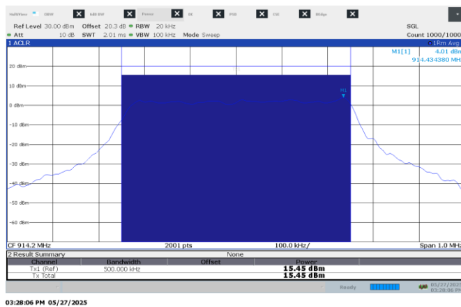
Figure 8.5-3: Output power on high channel, 500 kHz BW
