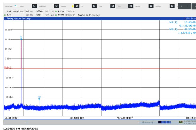
Figure 8.8-3: Conducted spurious emissions on high channel, 125 kHz BW
