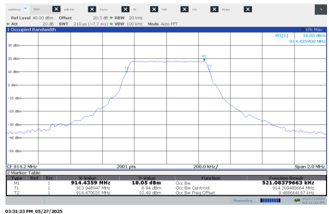
Figure 8.6-6: 99% occupied bandwidth sample plot – 500 kHz BW
