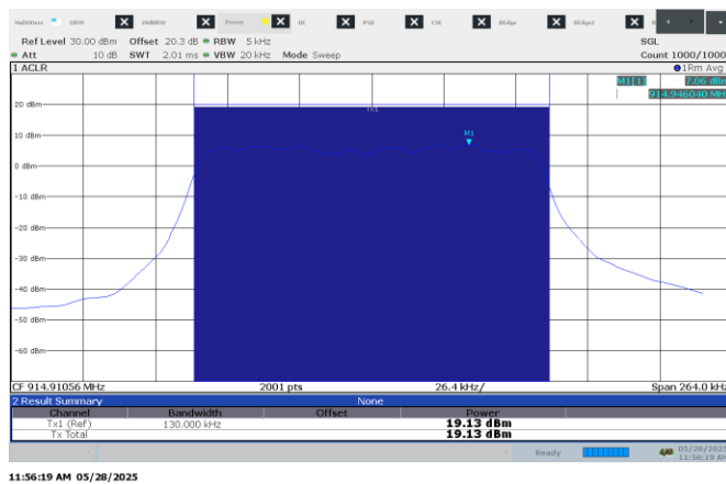
Figure 8.5-3: Output power on high channel, 125 kHz BW
