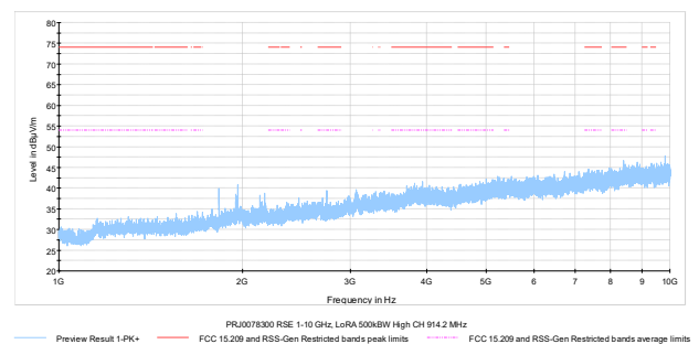
Figure 8.8-10: Radiated spurious emissions 1 – 10 GHz, LoRa 500 kHz BW, High channel 914.2 MHz
