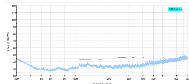
Figure 8.8-10: Radiated spurious emissions 30 – 1000 MHz, LoRa 125 kHz BW, High channel 914.9 MHz
