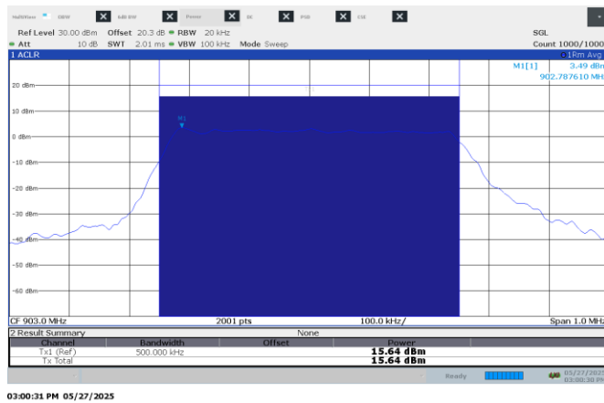
Figure 8.5-3: Output power on low channel, 500 kHz BW
