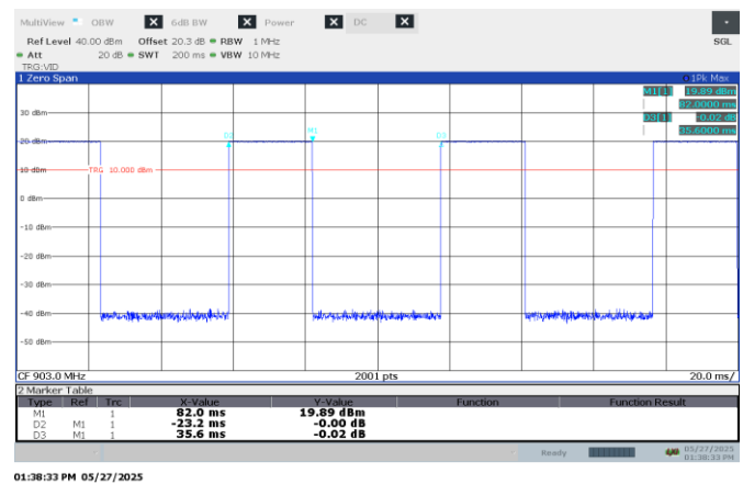
Figure 8.5-4: Duty cycle, 500 kHz BW
