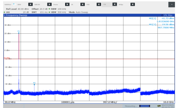
Figure 8.8-15: Conducted spurious emissions on mid channel, 500 kHz BW
