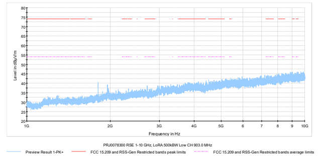
Figure 8.8-10: Radiated spurious emissions 1 – 10 GHz, LoRa 500 kHz BW, Low channel 903.0 MHz
