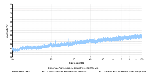
Figure 8.8-10: Radiated spurious emissions 1 – 10 GHz, LoRa 500 kHz BW, Mid channel 907.8 MHz
