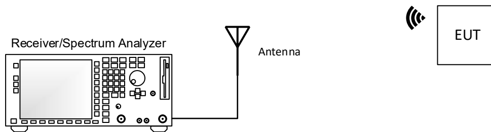
Figure 4.5-1: Radiated testing block diagram
