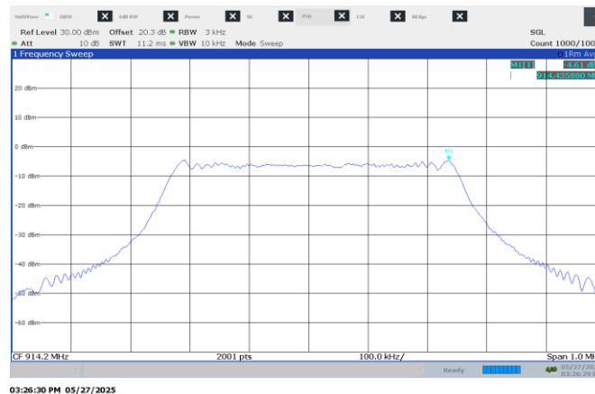
Figure 8.9-3: PSD on high channel, 500 kHz BW
