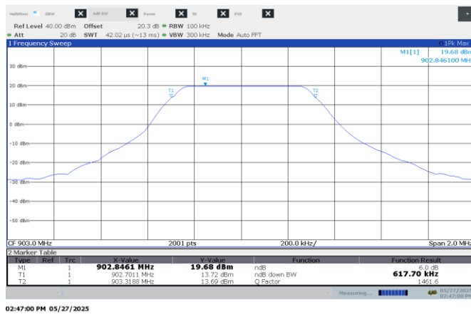
Figure 8.6-1: 6 dB bandwidth on Low channel – 500 kHz BW
