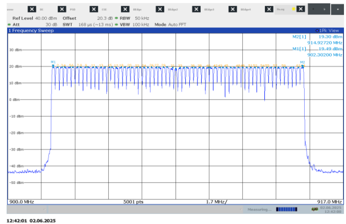
Figure 7.4-6: Number of hopping channels
