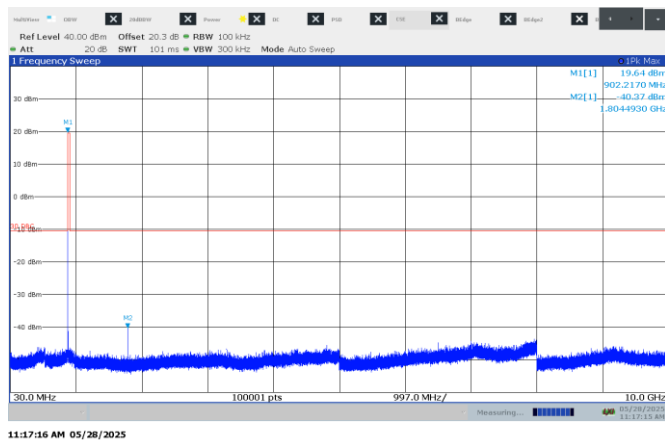
Figure 8.8-1: Conducted spurious emissions on low channel, 125 kHz BW
