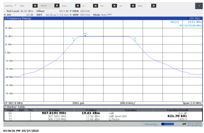
Figure 8.6-2: 6 dB bandwidth on Mid channel – 500 kHz BW
