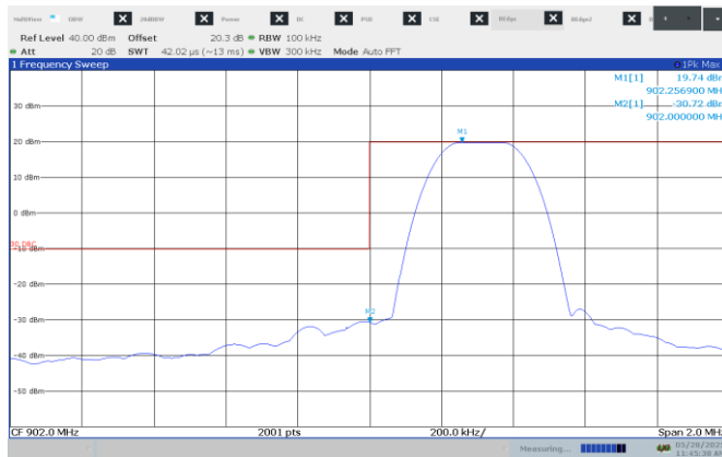
Figure 8.8-4: Conducted Band edge on low channel, 125 kHz BW
