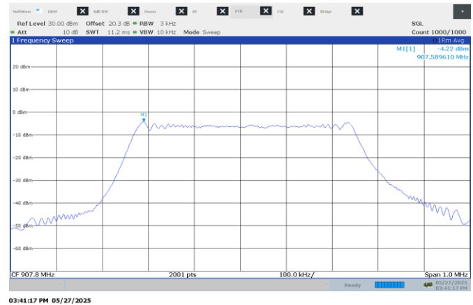
Figure 8.9-2: PSD on mid channel, 500 kHz BW
