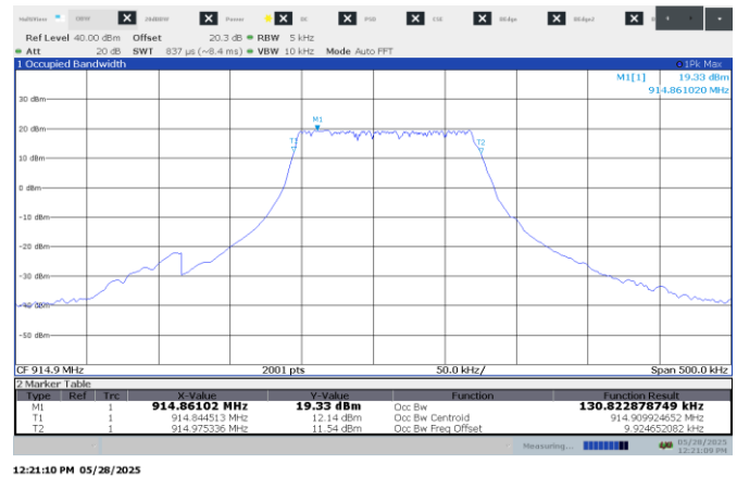
Figure 7.4-4: 99% occupied bandwidth sample plot – 125 kHz BW
