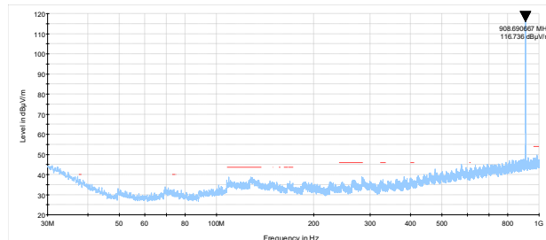
Figure 8.8-10: Radiated spurious emissions 30 – 1000 MHz, LoRa 125 kHz BW, Mid channel 908.7 MHz
