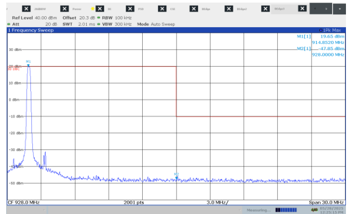
Figure 8.8-5: Conducted Band edge on high channel, 125 kHz BW
