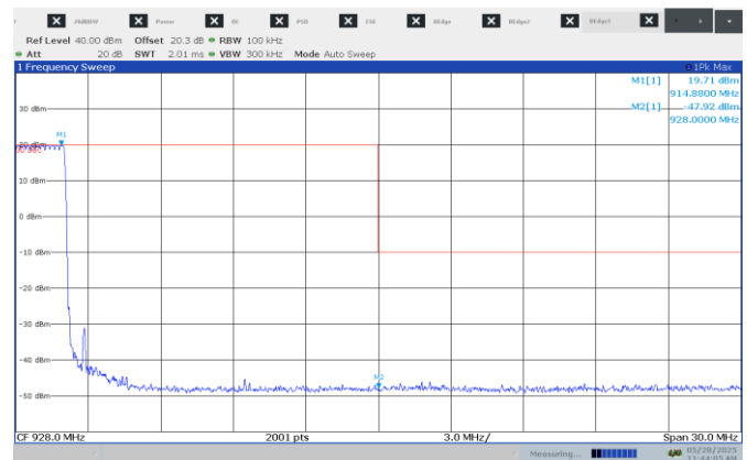
Figure 8.8-7: Conducted Band edge on high channel hopping, 125 kHz BW
