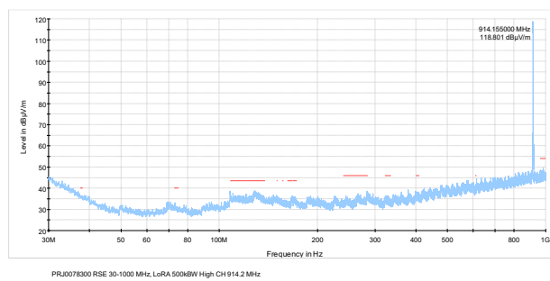
Figure 8.8-10: Radiated spurious emissions 30 – 1000 MHz, LoRa 500 kHz BW, High channel 914.2 MHz
