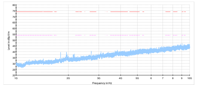
Figure 8.8-10: Radiated spurious emissions 1 – 10 GHz, LoRa 125 kHz BW, Low channel 902.3 MHz
