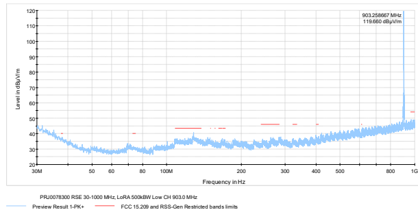
Figure 8.8-10: Radiated spurious emissions 30 – 1000 MHz, LoRa 500 kHz BW, Low channel 903.0 MHz
