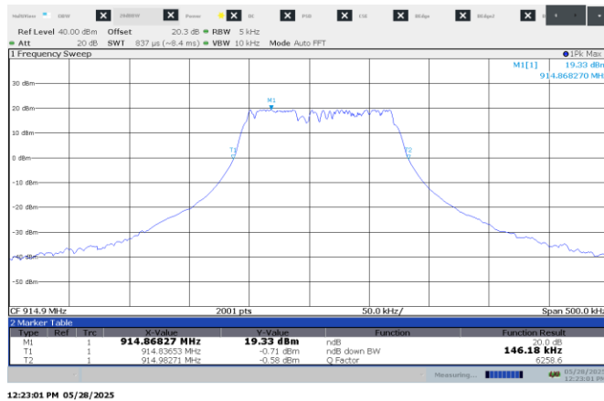
Figure 7.4-3: 20 dB bandwidth on high channel – 125 kHz BW
