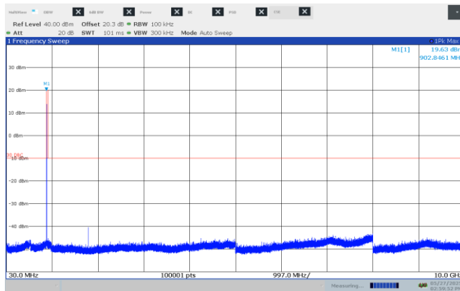
Figure 8.8-14: Conducted spurious emissions on low channel, 500 kHz BW
