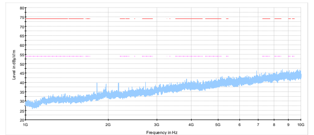
Figure 8.8-10: Radiated spurious emissions 1 – 10 GHz, LoRa 125 kHz BW, Mid channel 908.7 MHz
