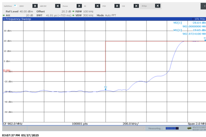
Figure 8.8-17: Conducted Band-edge on low channel, 500 kHz BW
