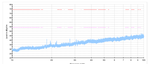
Figure 8.8-10: Radiated spurious emissions 1 – 10 GHz, LoRa 125 kHz BW, High channel 914.9 MHz
