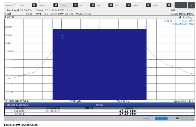
Figure 8.5-4: Output power on mid channel, 125 kHz BW
