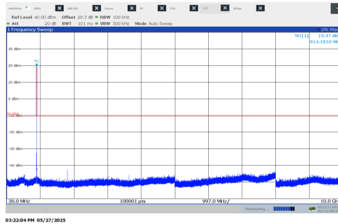
Figure 8.8-16: Conducted spurious emissions on high channel, 500 kHz BW
