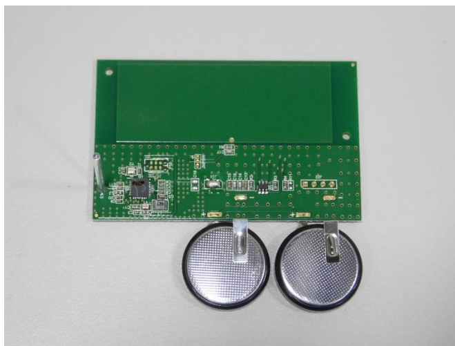
Figure 1.1-2: Bottom view of PCB
