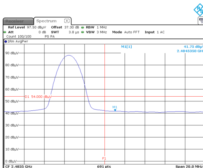
Figure 8.6-4: Radiated restricted upper band edge - Average
