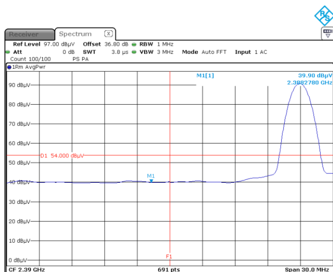
Figure 8.6-3: Radiated restricted lower band edge - Average
