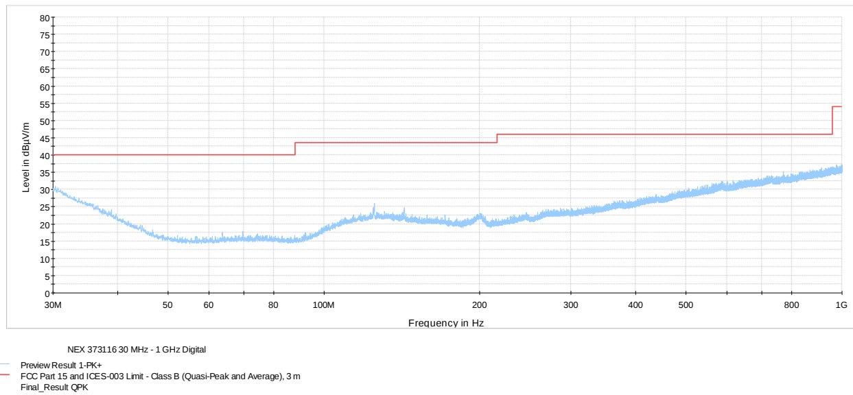
Figure 8.1-1: Radiated emissions spectral plot
