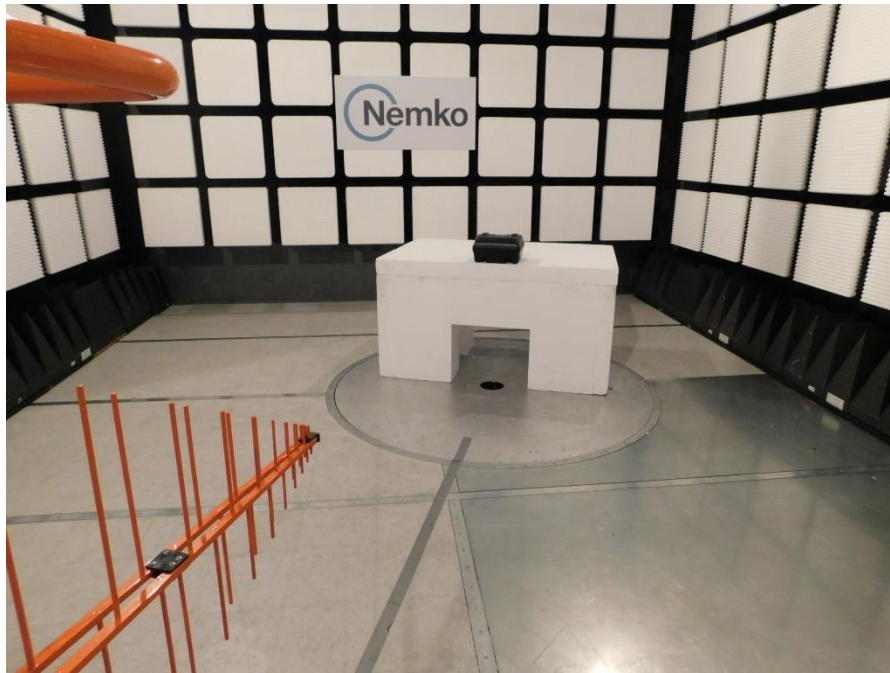
Figure 8.1-2: Radiated emissions setup photo - Front
