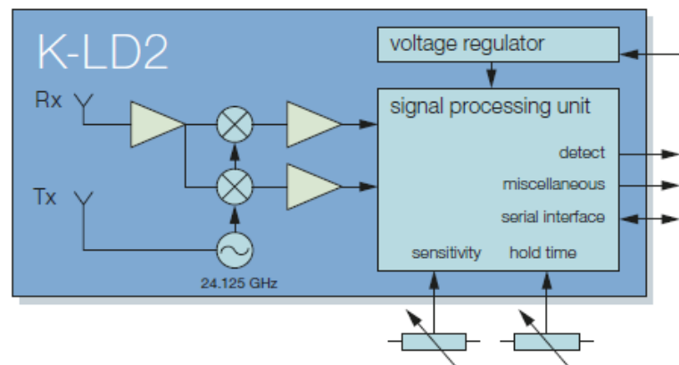
Figure 1: K-LD2 block diagram
