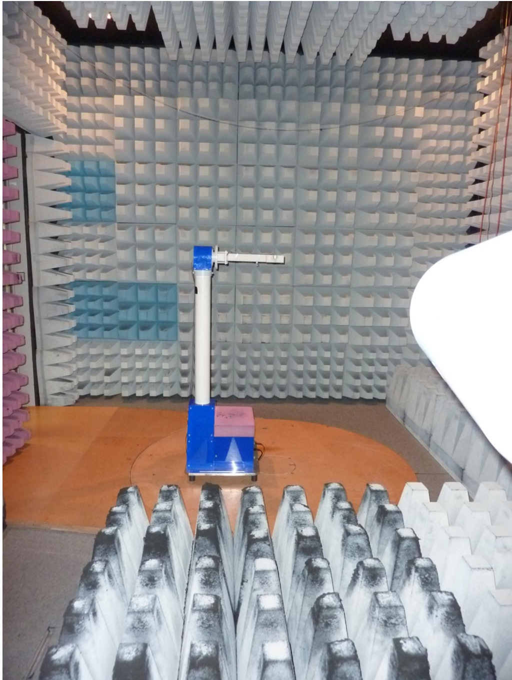
181710_m.jpg: K-LD2, test setup fully anechoic chamber
