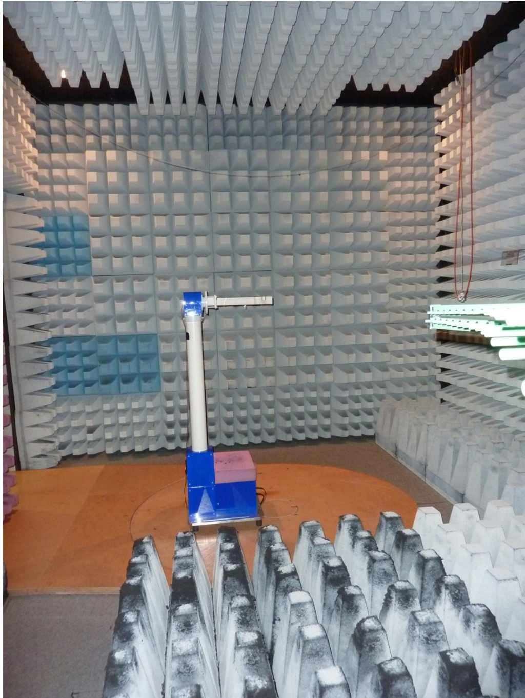
181710_l.jpg: K-LD2, test setup fully anechoic chamber
