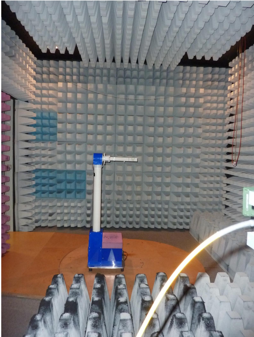
181710_p.jpg: K-LD2, test setup fully anechoic chamber
