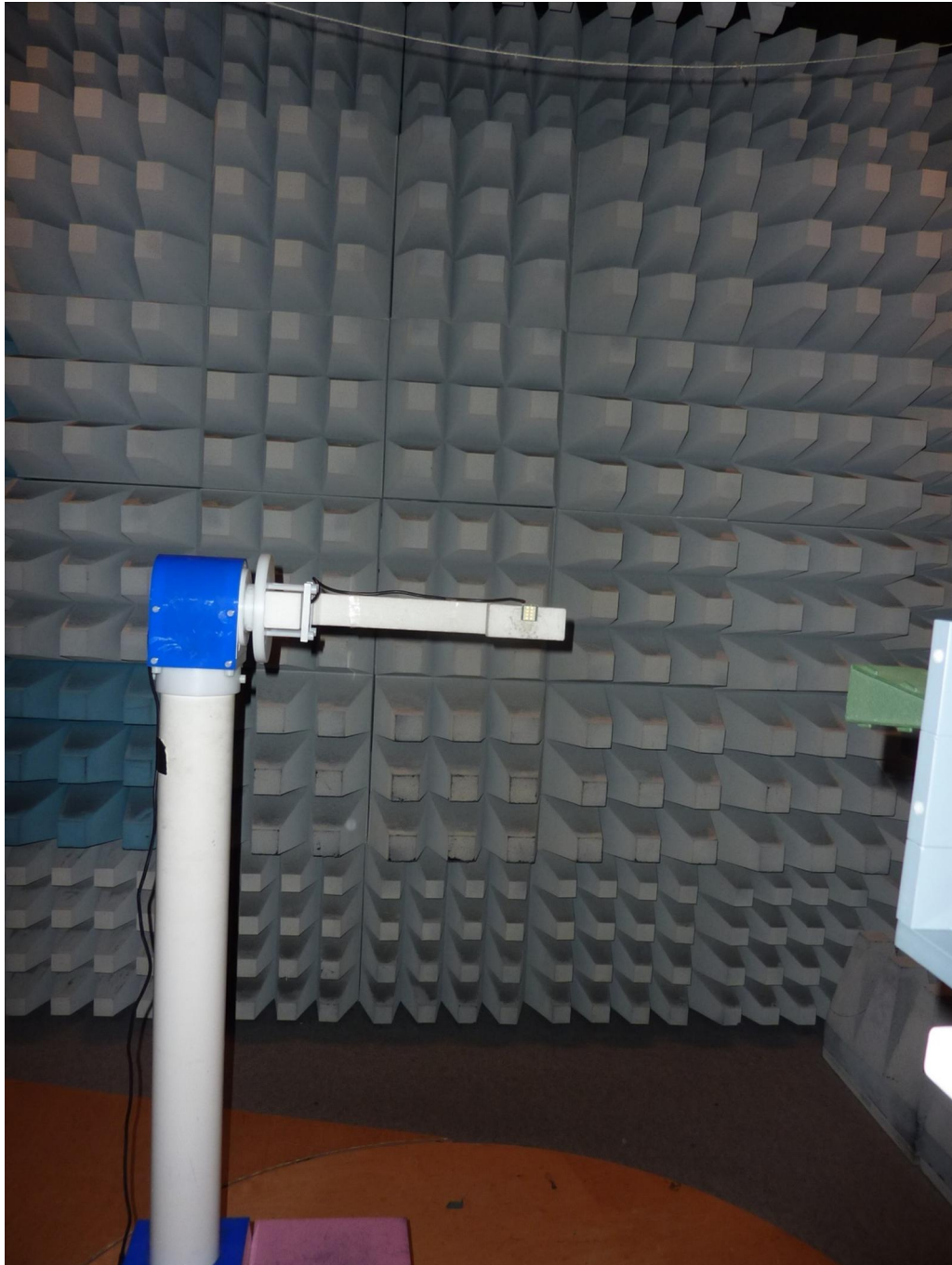
181710_n.jpg: K-LD2, test setup fully anechoic chamber
