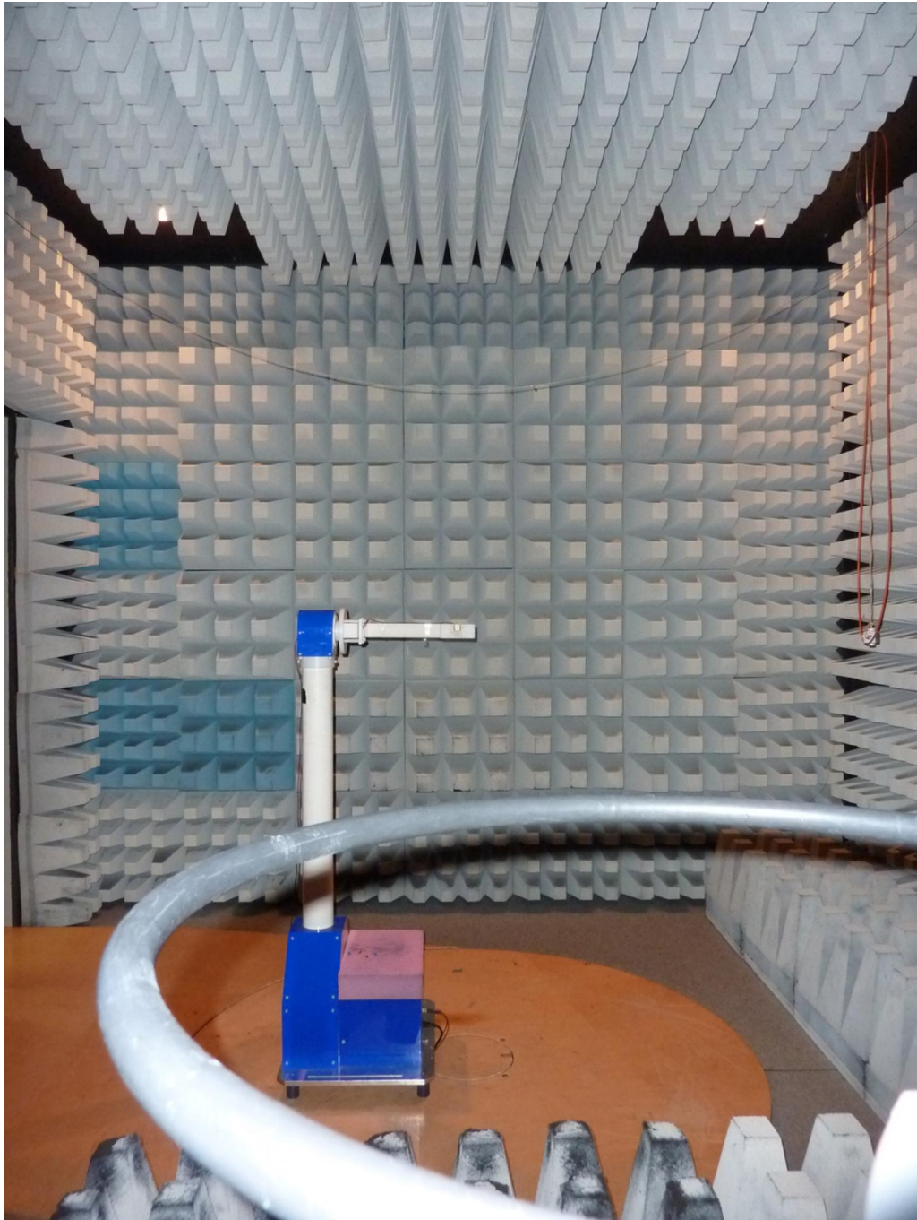
181710_k.jpg: K-LD2, test setup fully anechoic chamber
