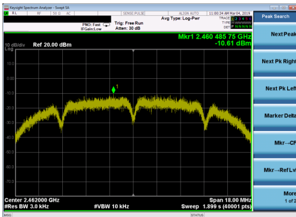
(802.11b) PSD plot on channel 11
