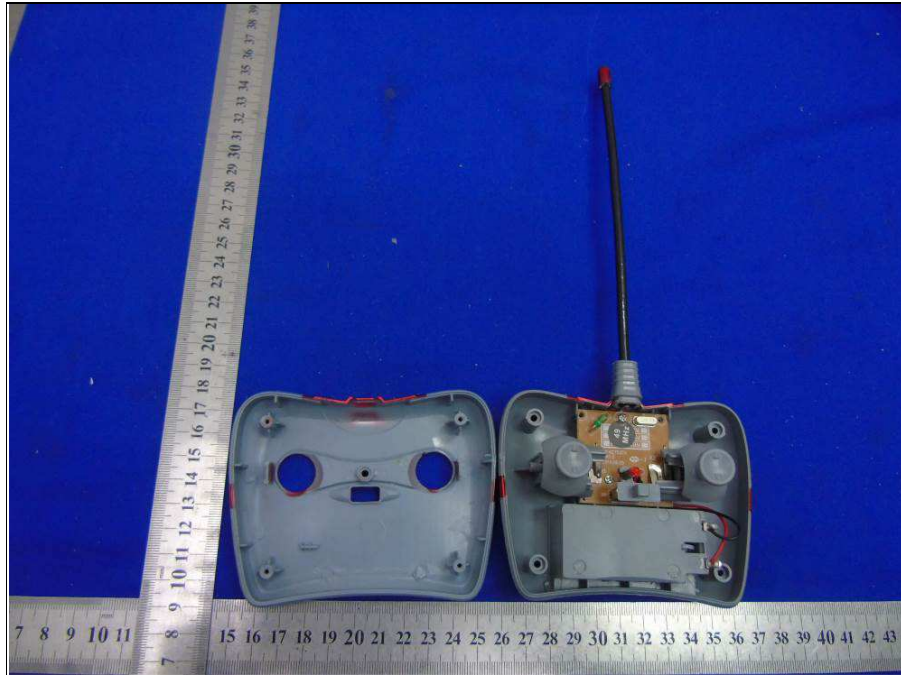
49.86MHz TX
