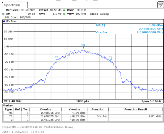
BLE_2M_High_Channel
