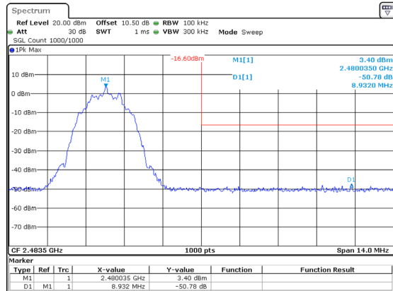
BLE_2M_High_Channel
