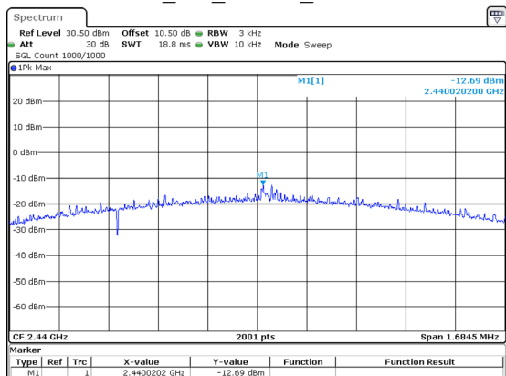
BLE_2M_Middle_Channel
