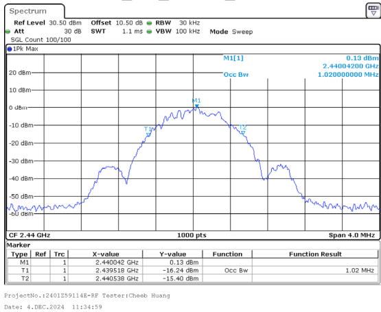
BLE_1M_Middle_Channel
