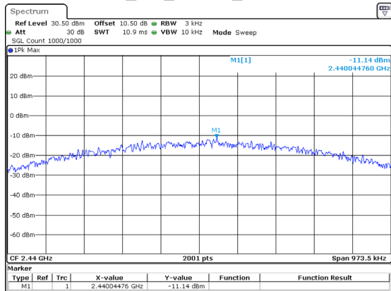
BLE_1M_Middle_Channel
