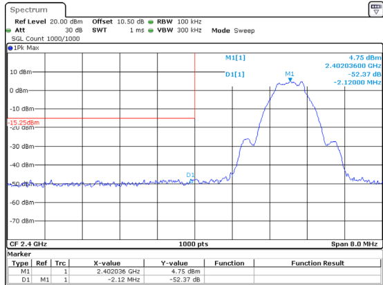
BLE_1M_Low_Channel
