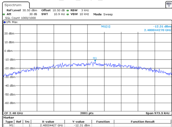
BLE_1M_High_Channel
