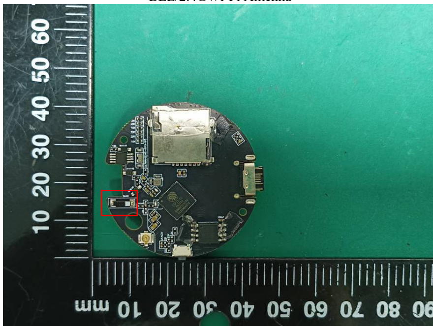
BLE/2.4GWi-Fi Antenna
