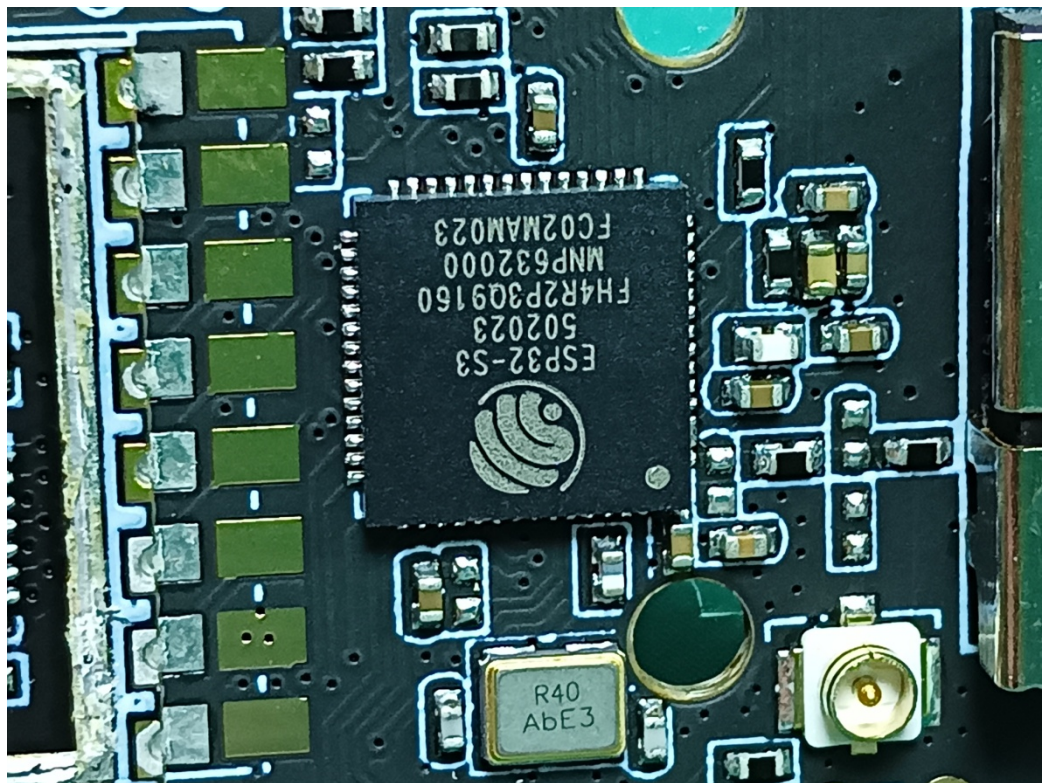
BLE/2.4GWi-Fi Antenna
