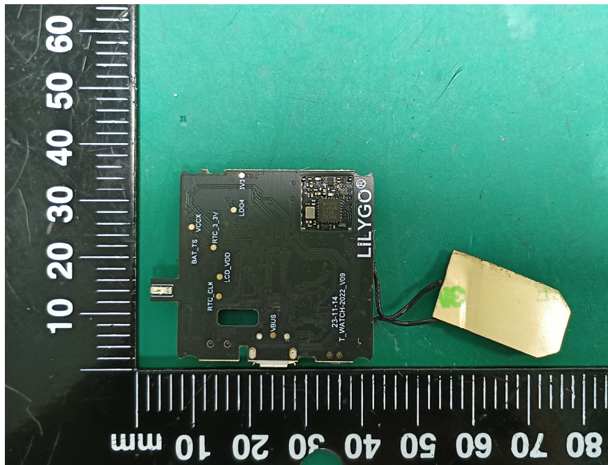
900M/BLE/Wi-Fi ANT
