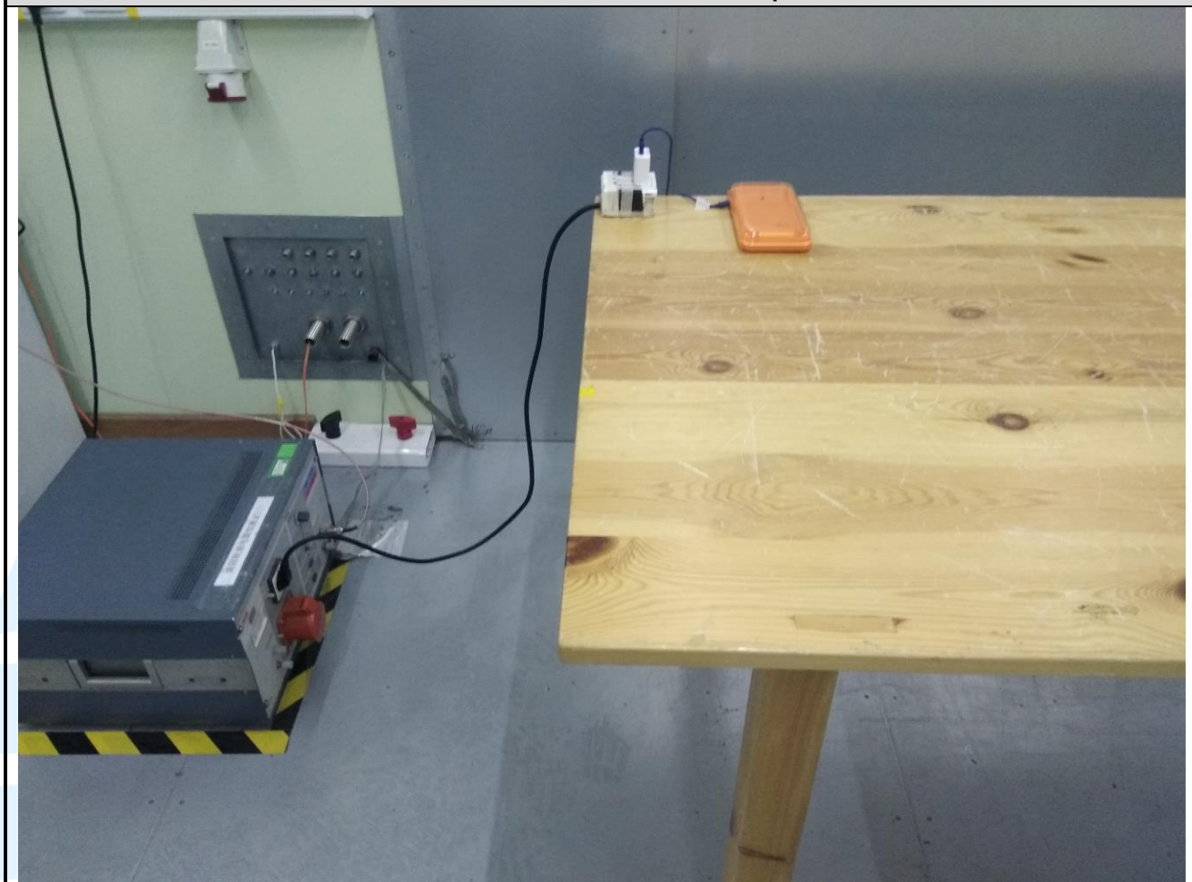
Conducted Emission Test Setup
