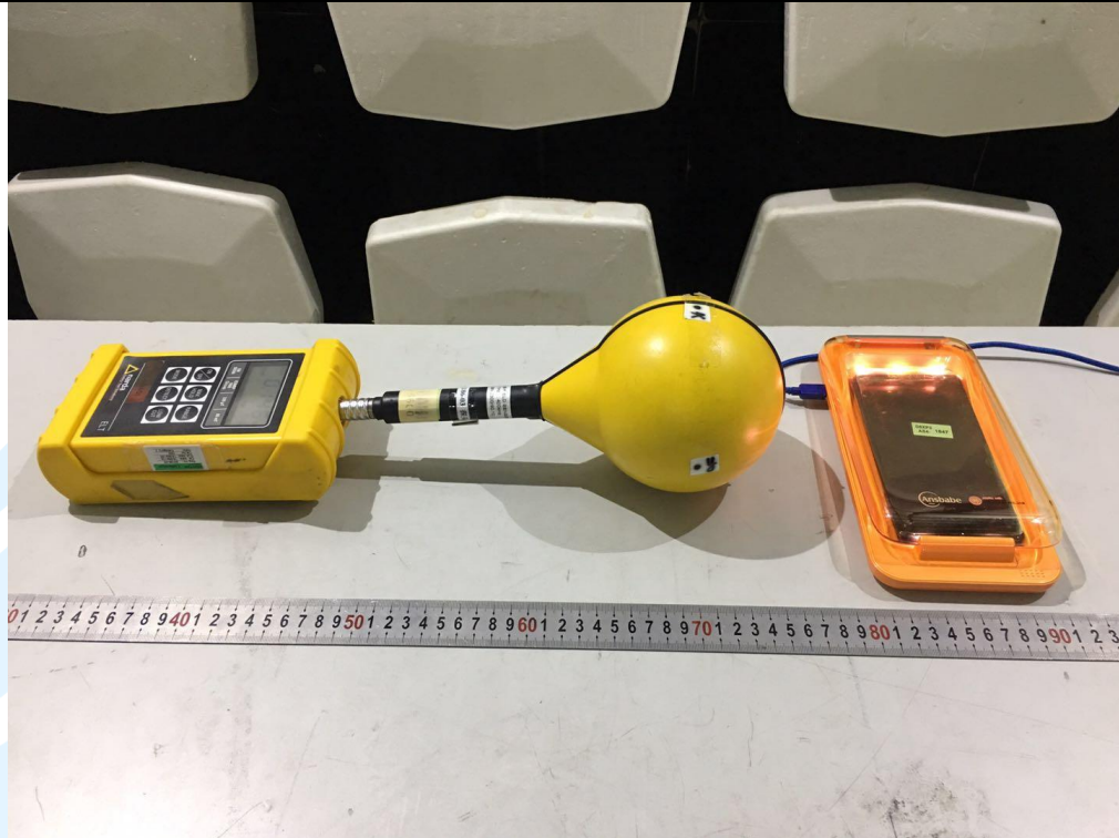
H-Field Strength position left
