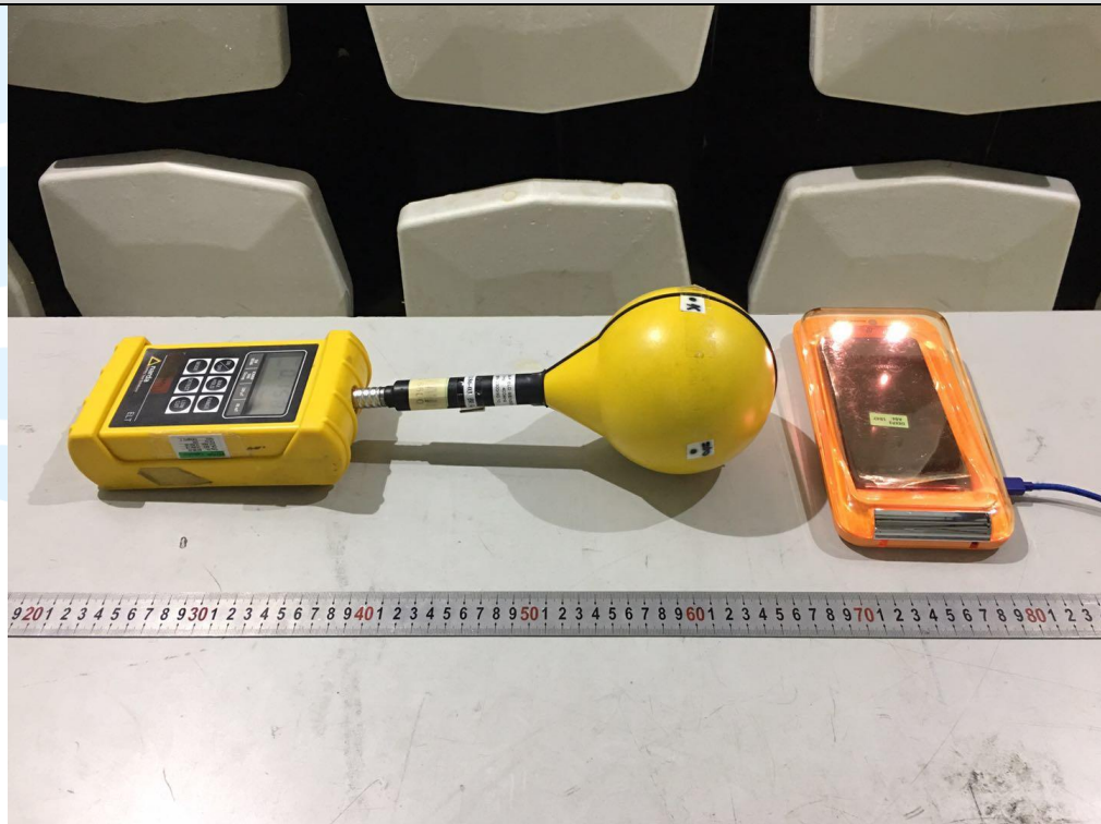
H-Field Strength position right
