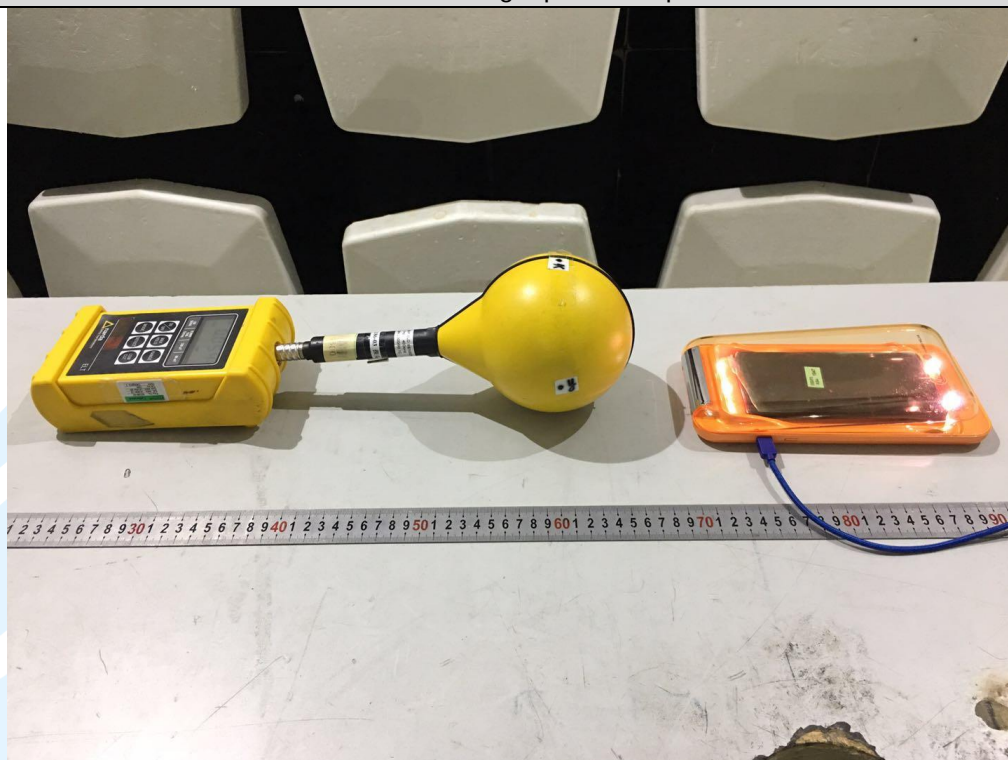
H-Field Strength position top
