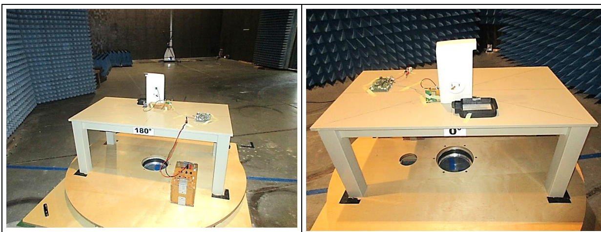
Fig 4 Spurious emissions 30 MHz – 1GHz
