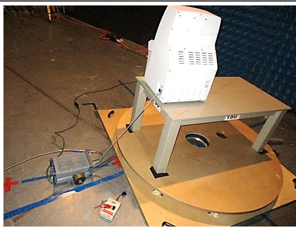
Fig 1 Conducted measurements – interference voltage
