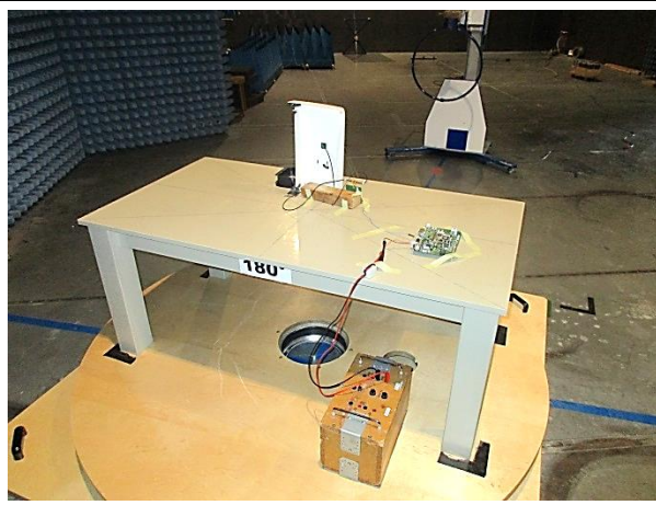
Fig 2 Radiated measurements – carrier, band edge and occupied bandwidth
