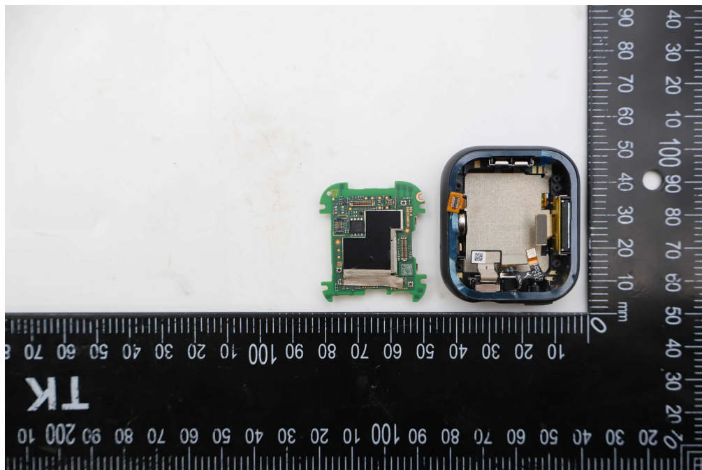
BT&Wi-Fi Antenna
