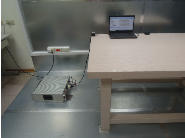
FCC_15_247_BLE_Conduction_Setup
