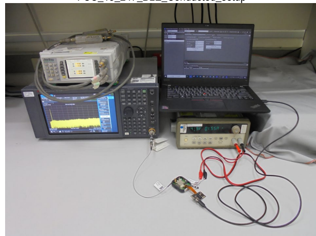
FCC_15_247_BLE_Conducted_setup
