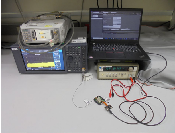
FCC_15_247_WLAN_Conducted_setup
