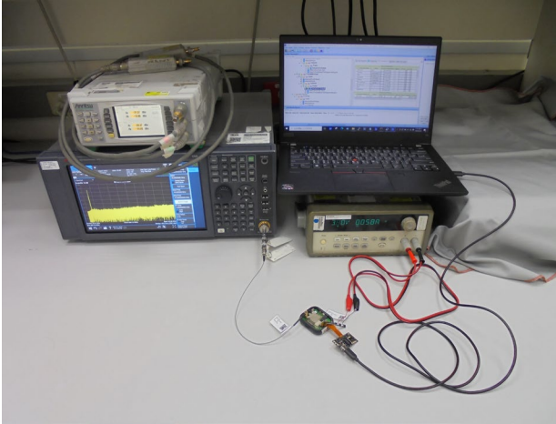
FCC_22_24_27_LTE_Conducted_Setup(1)
