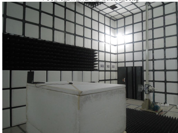
FCC_15_247_WLAN_Radiated_Setup
