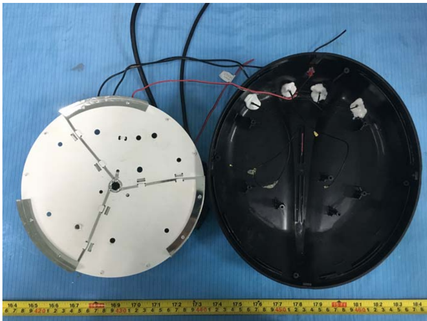
EUT – Cover off View 2 (Model: CA-1000 WIFI)
