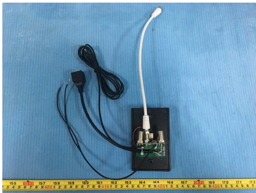
EUT – RF Splitter View 1
