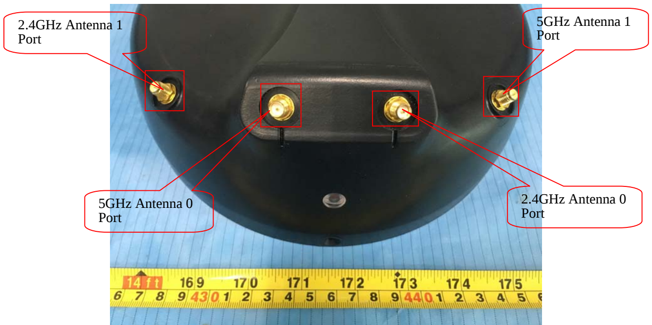
EUT – Antenna Port View
