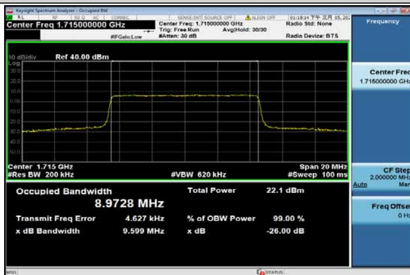
Band4-10MHz-16QAM-20175-50RB#0-8.9829
