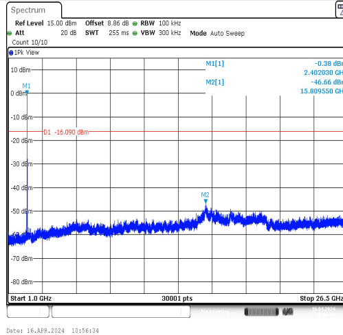
BLE_2M-Ant1-2402-1000~26500-PASS
