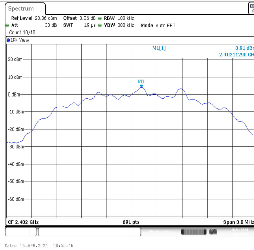
BLE_2M-Ant1-2402-0~Reference-PASS
