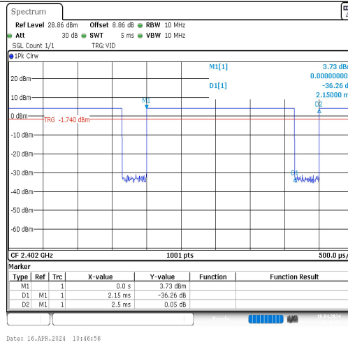
NTNV-BLE_1M-Ant1-2402
