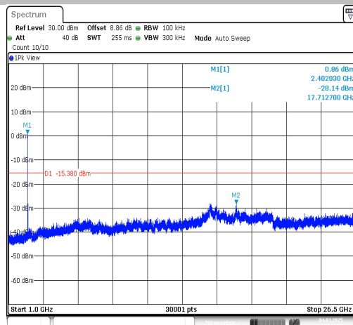
BLE_2M-Ant1-2402-0~Reference-PASS
