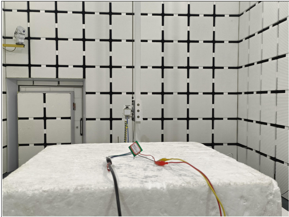
RADIATED EMISSION TEST (18GHz ~ 25GHz)
