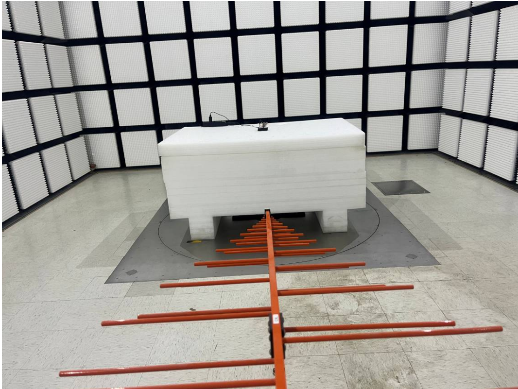
Radiated Emission Below 1GHz View (Adapter)
