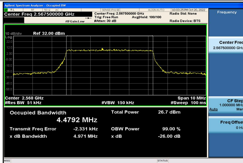
Band7-5MHz-16QAM-21425-25RB#0-4.4792
