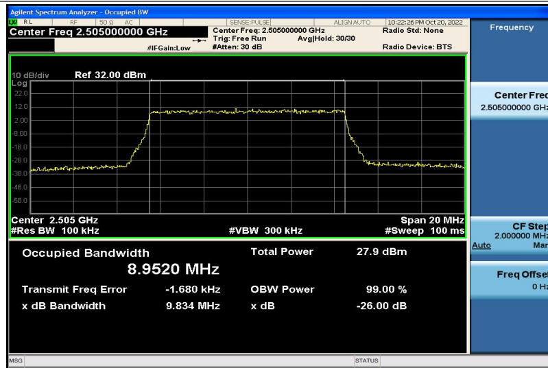
Band7-10MHz-16QAM-20800-50RB#0-8.9520
