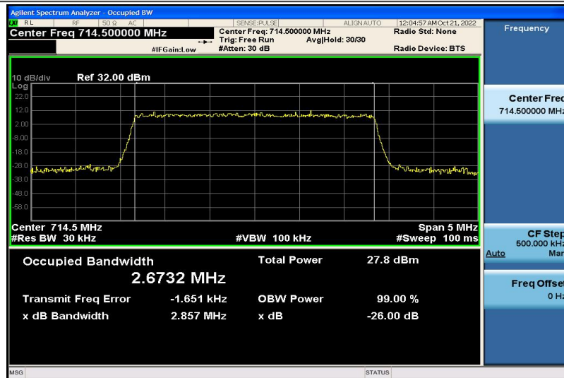
Band12-3MHz-16QAM-23165-15RB#0-2.6732
