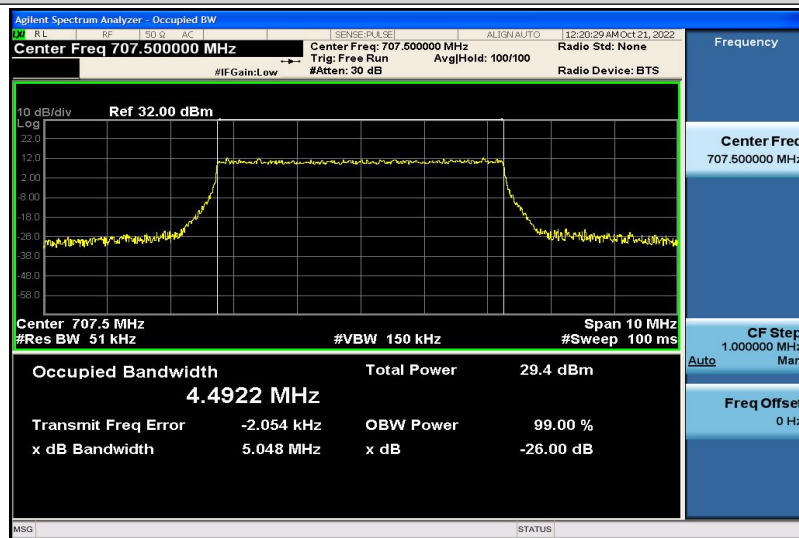
Band12-5MHz-QPSK-23095-25RB#0-4.4922
