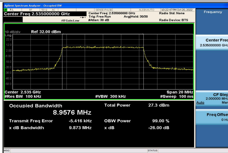
Band7-10MHz-16QAM-21100-50RB#0-8.9576
