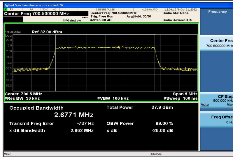
Band12-3MHz-16QAM-23025-15RB#0-2.6771
