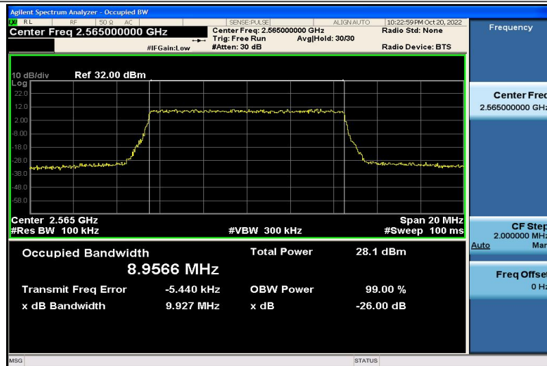
Band7-10MHz-QPSK-21400-50RB#0-8.9566
