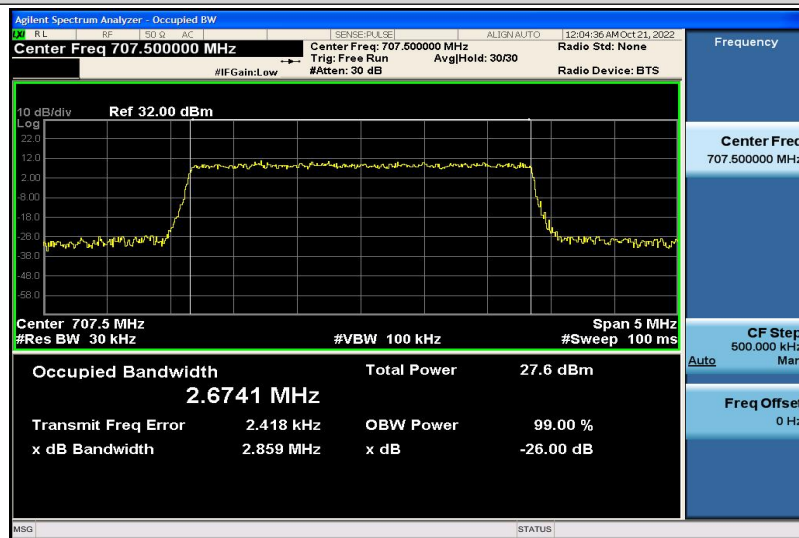
Band12-3MHz-16QAM-23095-15RB#0-2.6741
