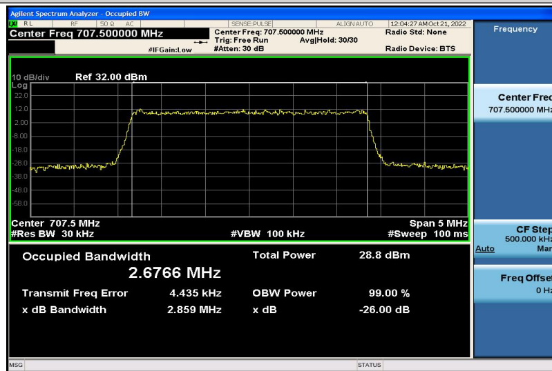
Band12-3MHz-QPSK-23095-15RB#0-2.6766
