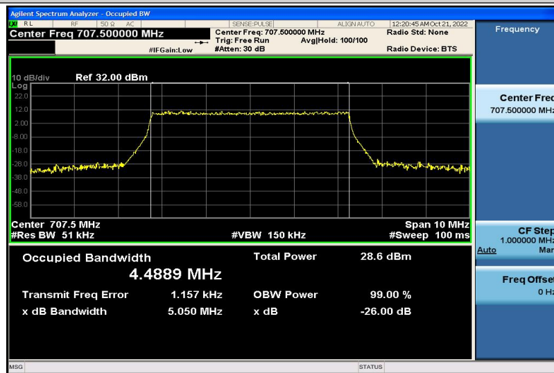
Band12-5MHz-16QAM-23095-25RB#0-4.4889
