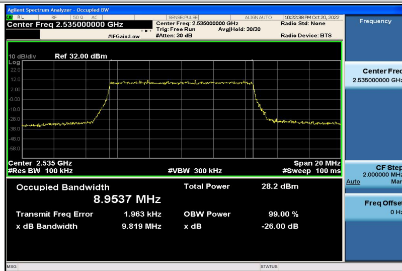
Band7-10MHz-QPSK-21100-50RB#0-8.9537
