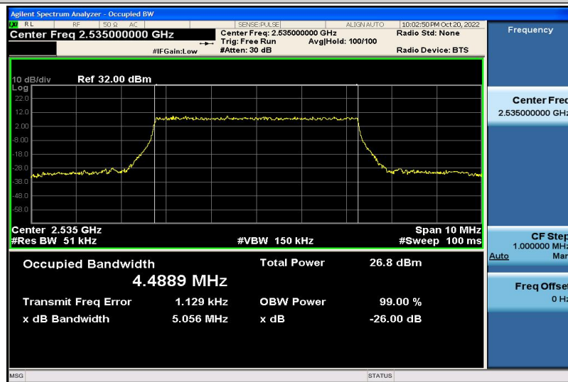
Band7-5MHz-16QAM-21100-25RB#0-4.4889
