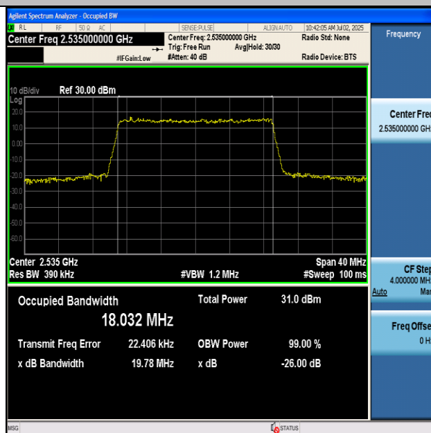
Band7-20MHz-16QAM-21100-100RB#0-PASS
