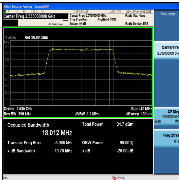
Band7-20MHz-QPSK-21100-100RB#0-PASS
