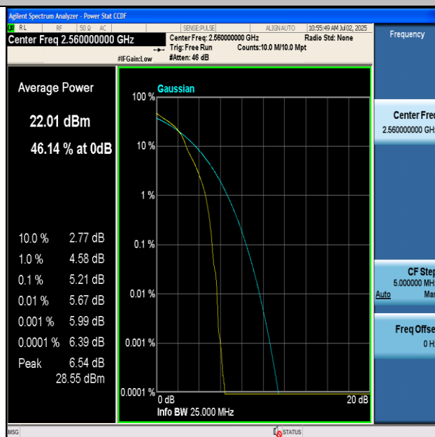
Band7-20MHz-16QAM-21350-1RB#0-PASS
