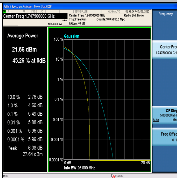
Band4-15MHz-16QAM-20325-1RB#0-PASS
