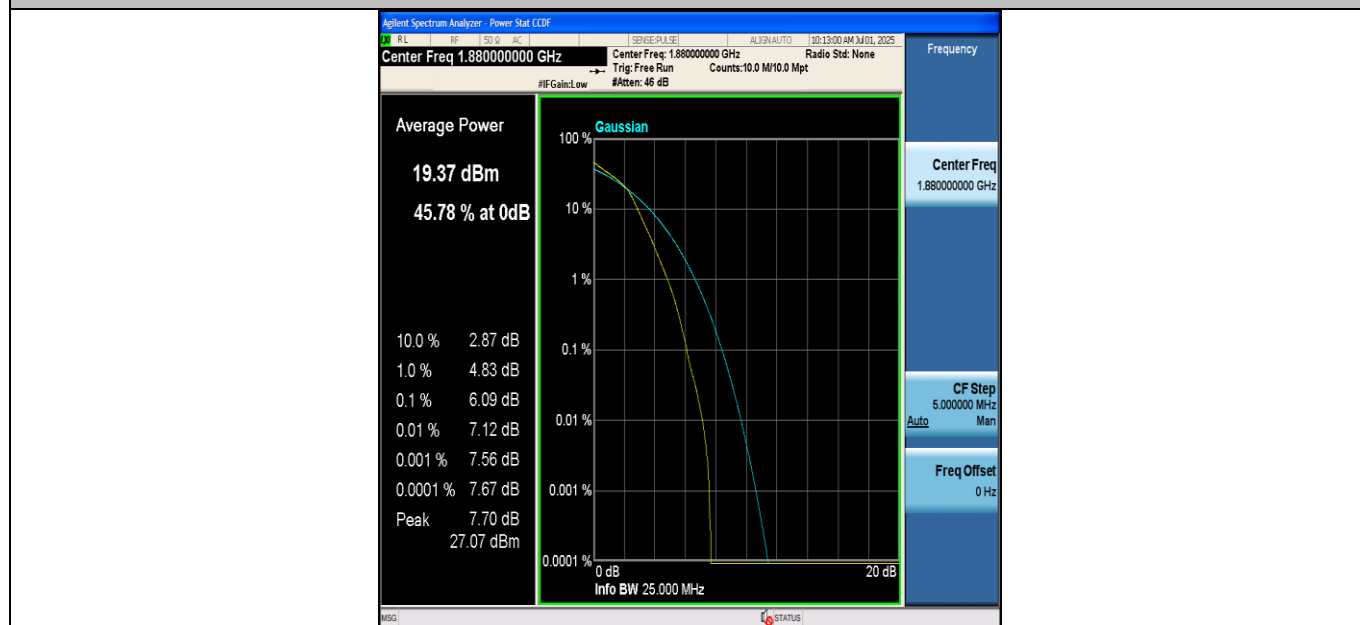
Band2-1.4MHz-16QAM-18900-6RB#0-PASS
