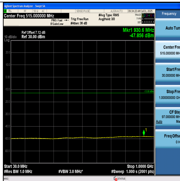
Band2-9400-30~1000MHz-PASS
