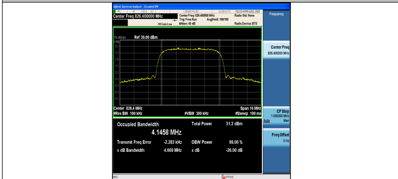
Band5-4132-PASS
