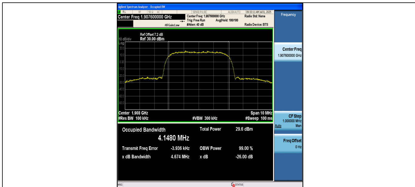
Band2-9538-PASS
