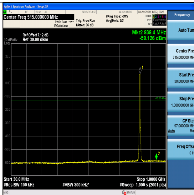
Band5-4182-30~1000MHz-PASS
