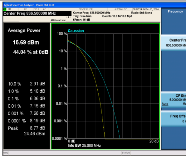
Band5-5MHz-16QAM-20525-25RB#0-PASS
