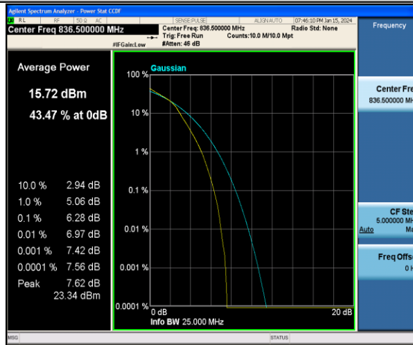
Band5-3MHz-16QAM-20525-15RB#0-PASS
