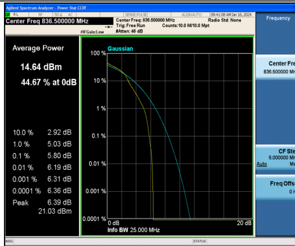
Band5-10MHz-16QAM-20525-1RB#0-PASS
