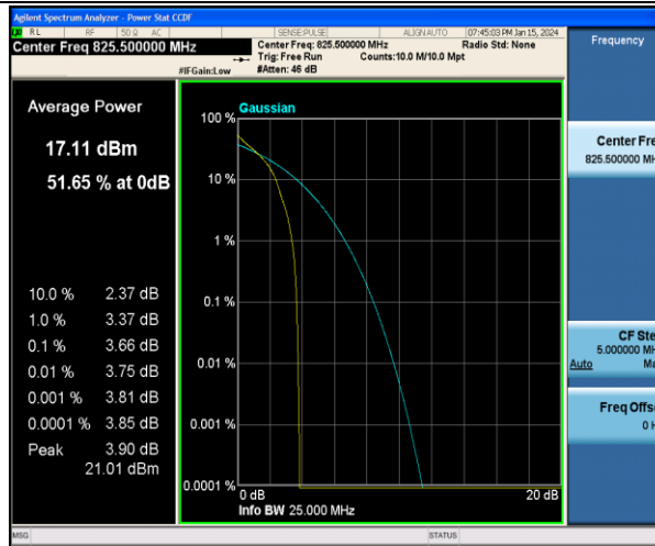
Band5-3MHz-QPSK-20415-1RB#0-PASS
