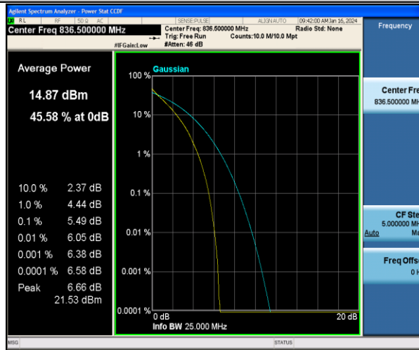
Band5-10MHz-QPSK-20525-50RB#0-PASS
