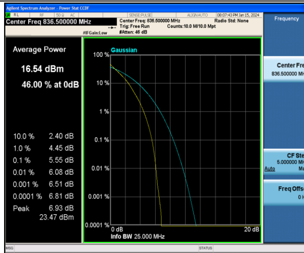
Band5-5MHz-QPSK-20525-25RB#0-PASS
