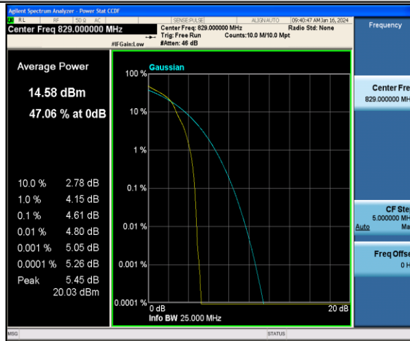
Band5-10MHz-16QAM-20450-1RB#0-PASS
