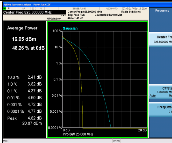
Band5-3MHz-QPSK-20415-15RB#0-PASS
