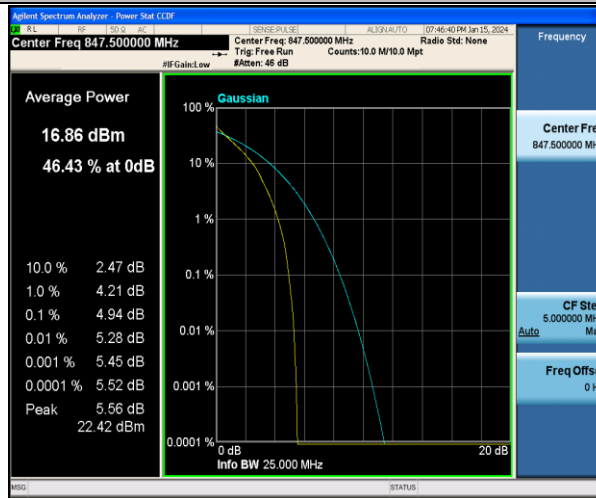
Band5-3MHz-QPSK-20635-15RB#0-PASS
