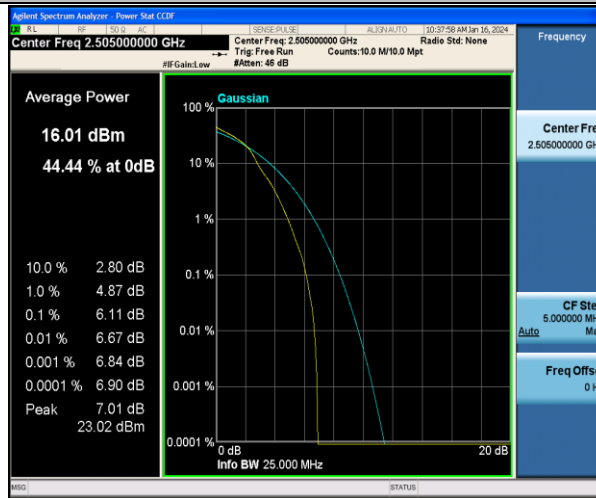
Band7-10MHz-16QAM-20800-1RB#0-PASS
