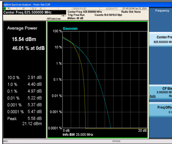
Band5-3MHz-16QAM-20415-15RB#0-PASS
