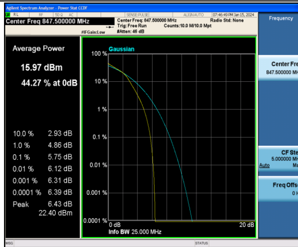
Band5-3MHz-16QAM-20635-15RB#0-PASS
