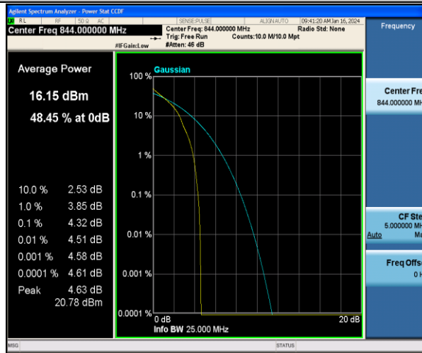
Band5-10MHz-QPSK-20600-1RB#0-PASS
