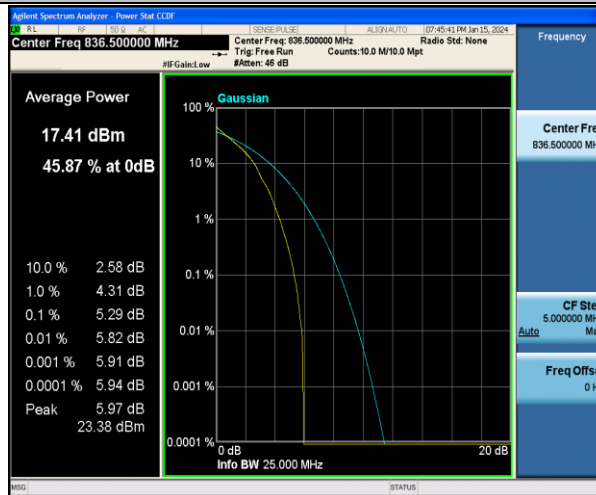
Band5-3MHz-QPSK-20525-1RB#0-PASS
