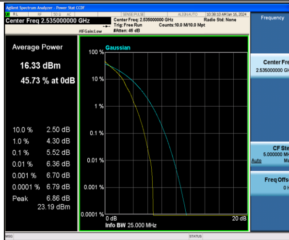
Band7-10MHz-QPSK-21100-1RB#0-PASS
