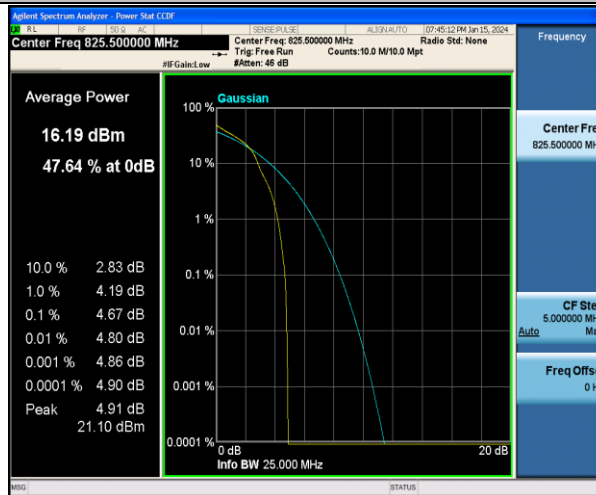
Band5-3MHz-16QAM-20415-1RB#0-PASS
