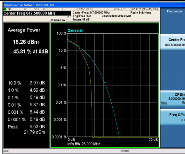
Band5-3MHz-16QAM-20635-1RB#0-PASS
