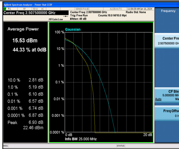
Band7-15MHz-16QAM-20825-1RB#0-PASS
