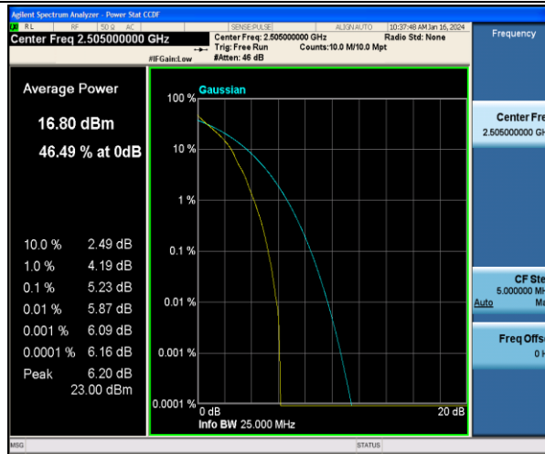
Band7-10MHz-QPSK-20800-1RB#0-PASS
