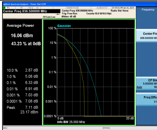
Band5-3MHz-16QAM-20525-1RB#0-PASS
