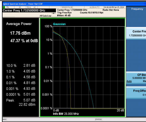
Band4-3MHz-16QAM-20175-15RB#0-PASS
