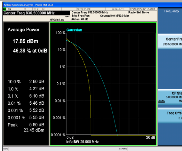
Band5-1.4MHz-QPSK-20525-1RB#0-PASS
