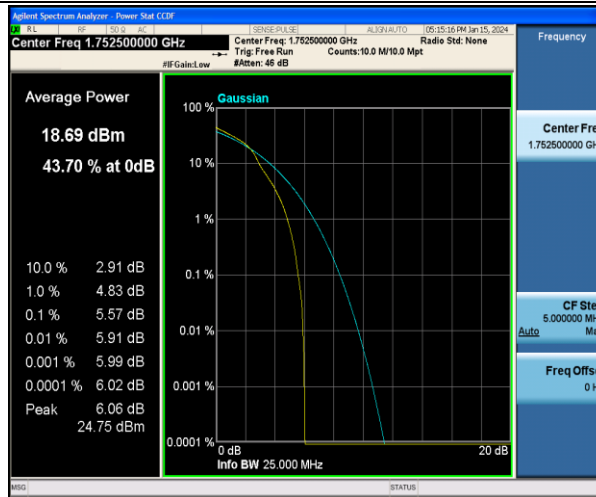
Band4-5MHz-16QAM-20375-1RB#0-PASS
