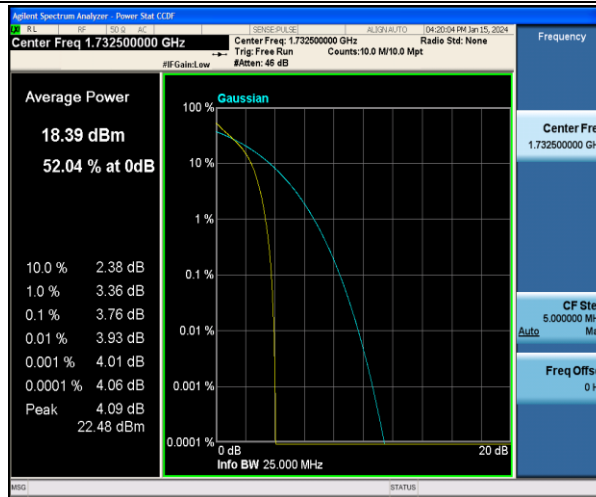
Band4-1.4MHz-QPSK-20175-6RB#0-PASS
