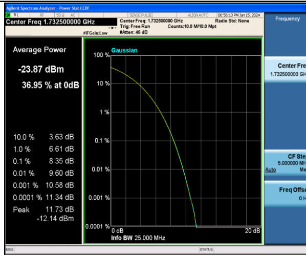
Band4-20MHz-QPSK-20175-100RB#0-PASS
