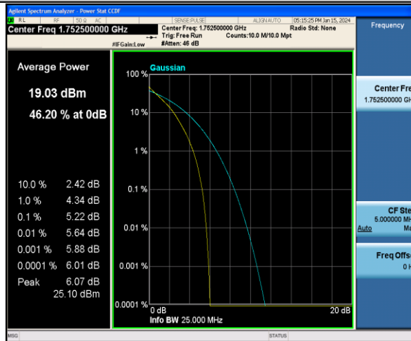
Band4-5MHz-QPSK-20375-25RB#0-PASS
