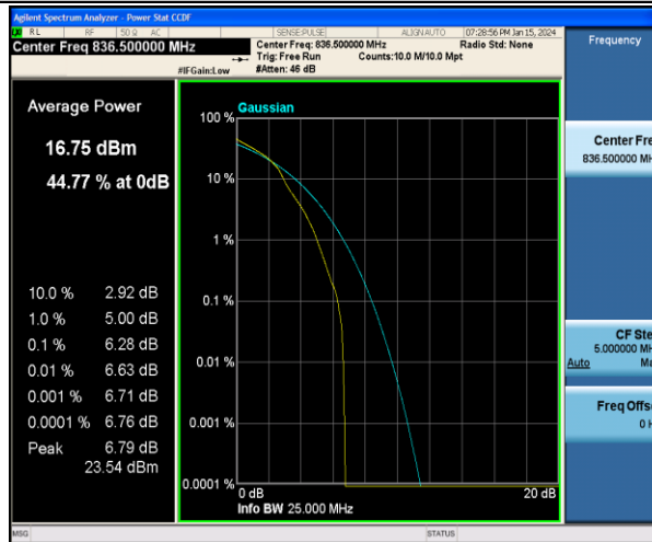
Band5-1.4MHz-16QAM-20525-1RB#0-PASS
