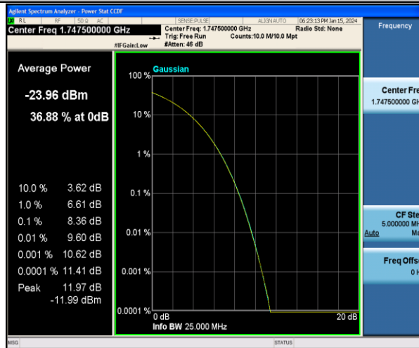
Band4-15MHz-QPSK-20325-1RB#0-PASS
