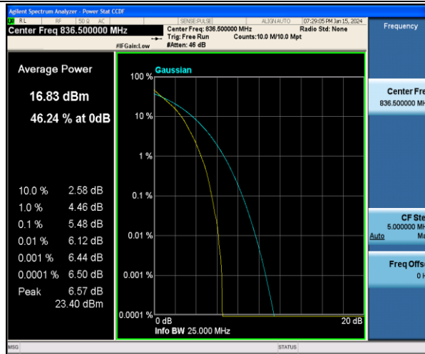
Band5-1.4MHz-QPSK-20525-6RB#0-PASS
