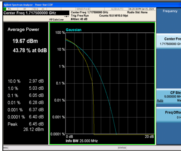
Band4-15MHz-16QAM-20025-1RB#0-PASS
