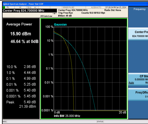
Band5-1.4MHz-16QAM-20407-6RB#0-PASS
