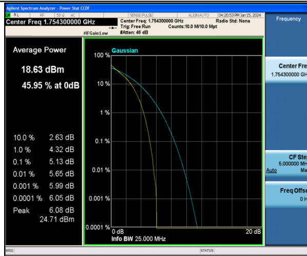
Band4-1.4MHz-QPSK-20393-6RB#0-PASS
