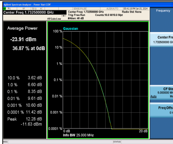
Band4-10MHz-QPSK-20175-1RB#0-PASS
