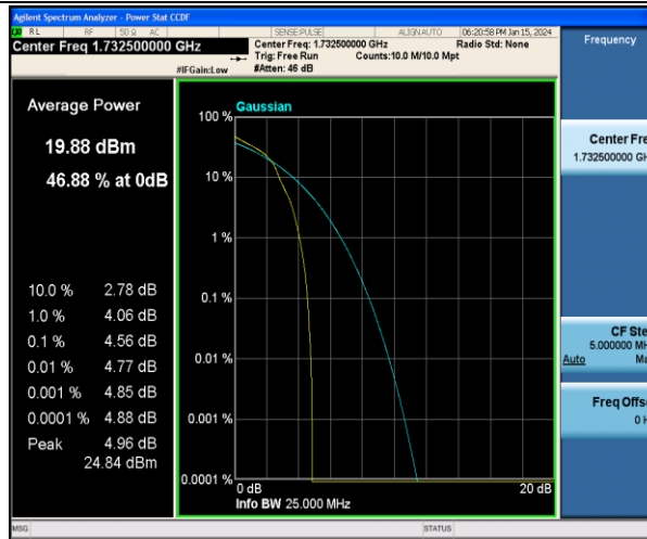
Band4-15MHz-16QAM-20175-1RB#0-PASS
