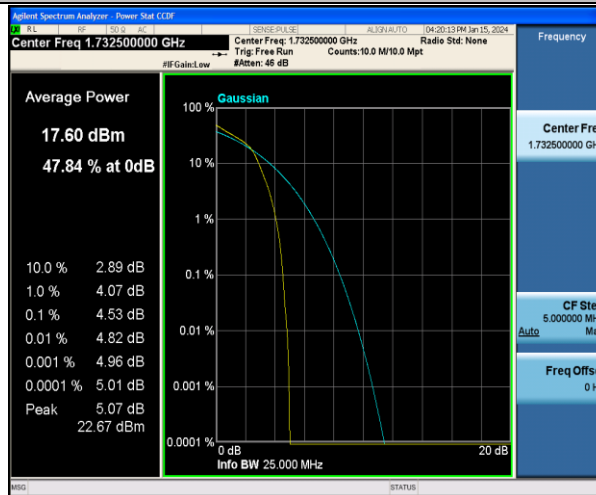
Band4-1.4MHz-16QAM-20175-6RB#0-PASS
