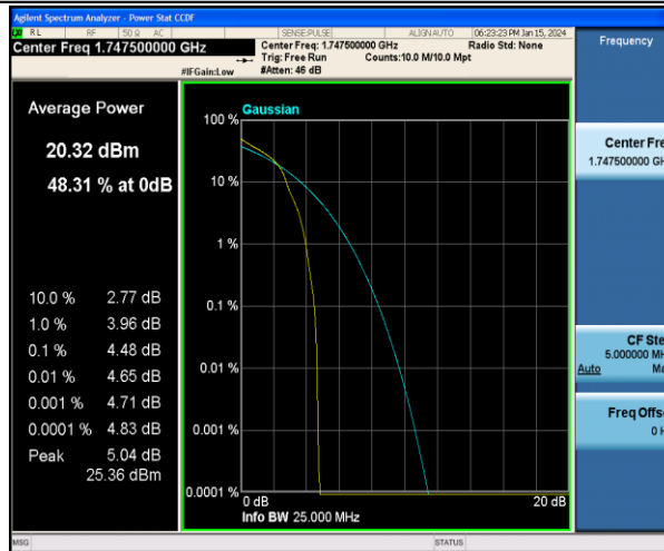
Band4-15MHz-16QAM-20325-1RB#0-PASS
