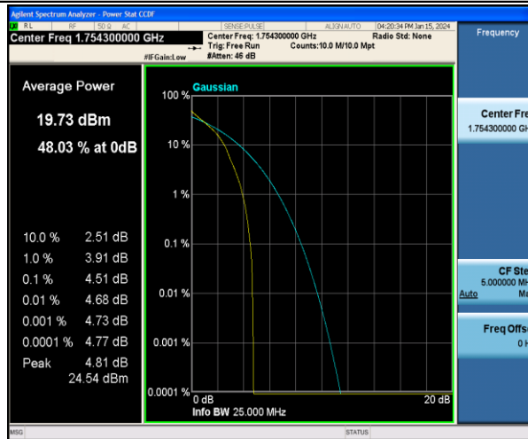
Band4-1.4MHz-QPSK-20393-1RB#0-PASS
