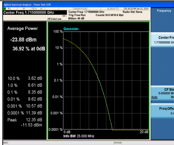
Band4-10MHz-16QAM-20000-1RB#0-PASS
