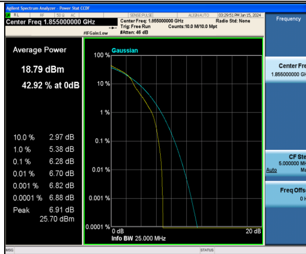
Band2-10MHz-16QAM-18650-1RB#0-PASS
