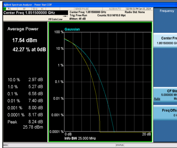
Band2-3MHz-16QAM-18615-15RB#0-PASS
