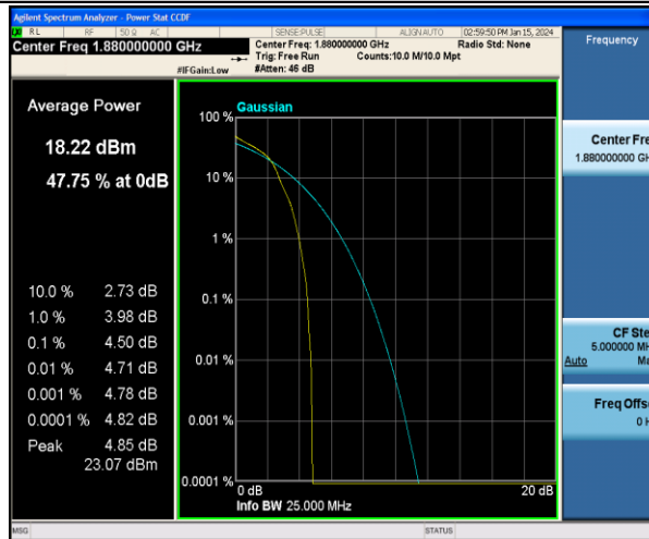
Band2-3MHz-16QAM-18900-1RB#0-PASS
