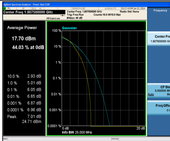
Band2-5MHz-16QAM-19175-25RB#0-PASS
