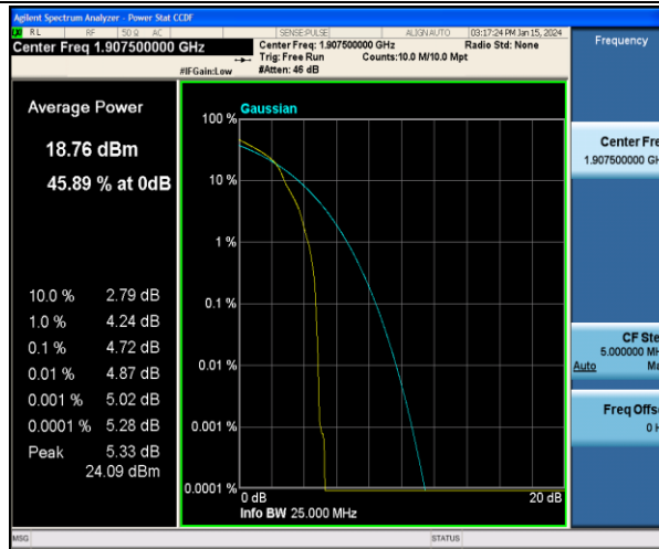
Band2-5MHz-16QAM-19175-1RB#0-PASS
