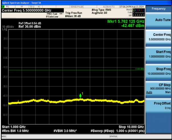
Band5_10MHz_16QAM_20525_1RB#0_1000~10000_1000~10000
