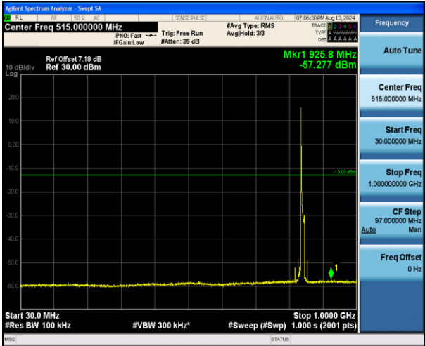
Band5_10MHz_QPSK_20600_1RB#0_30~1000_30~1000
