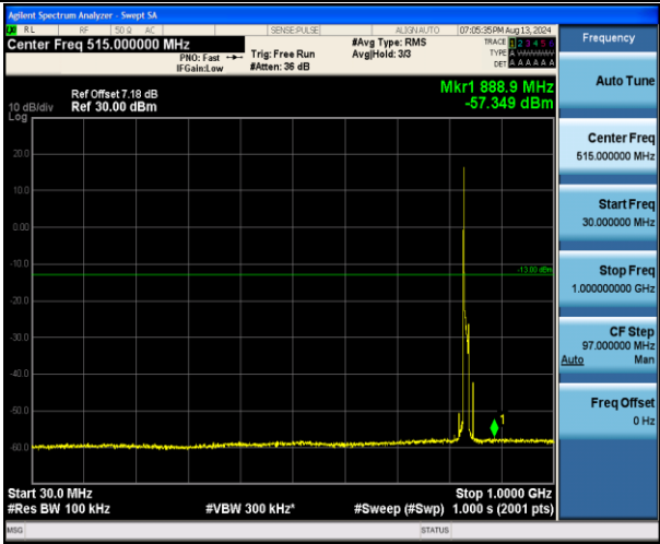
Band5_10MHz_QPSK_20525_1RB#0_30~1000_30~1000
