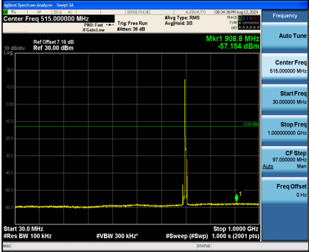
Band17_5MHz_16QAM_23755_1RB#0_30~1000_30~1000
