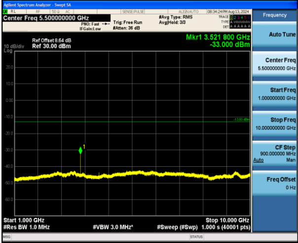
Band17_5MHz_QPSK_23755_1RB#0_1000~10000_1000~10000
