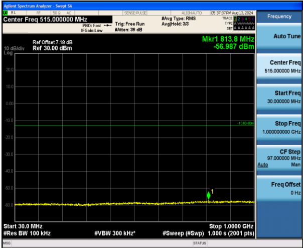
Band4_15MHz_QPSK_20325_1RB#0_30~1000_30~1000
