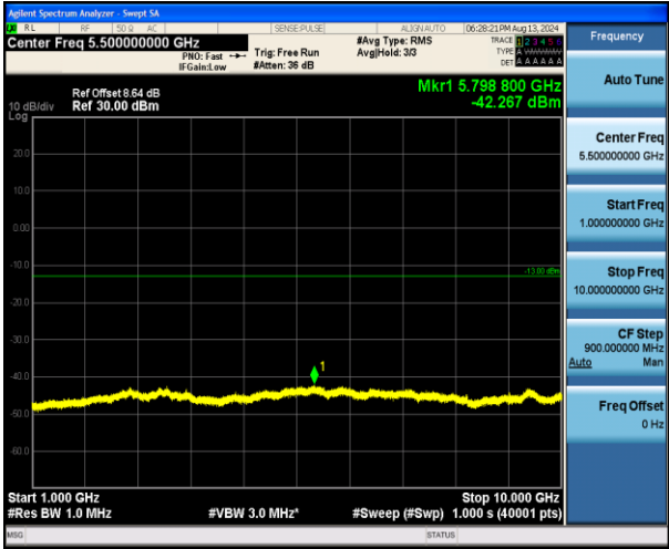
Band5_3MHz_QPSK_20415_1RB#0_1000~10000_1000~10000
