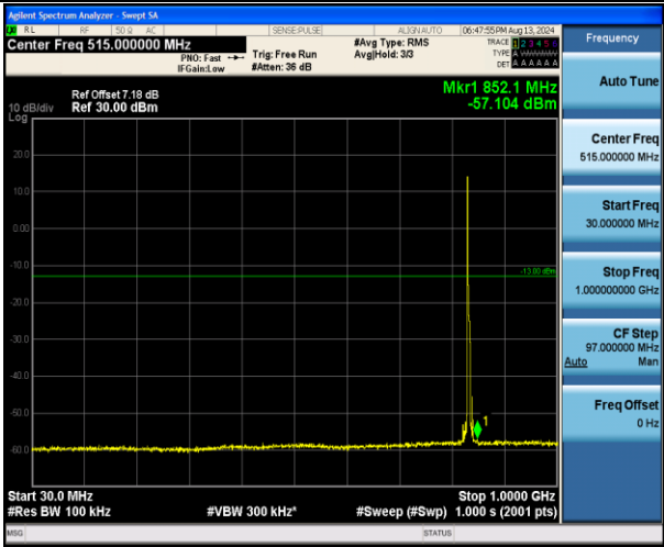
Band5_5MHz_QPSK_20525_1RB#0_30~1000_30~1000
