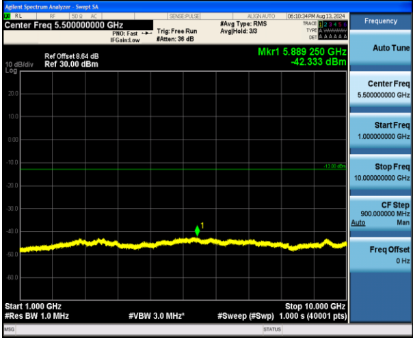
Band5_1.4MHz_QPSK_20407_1RB#0_1000~10000_1000~10000
