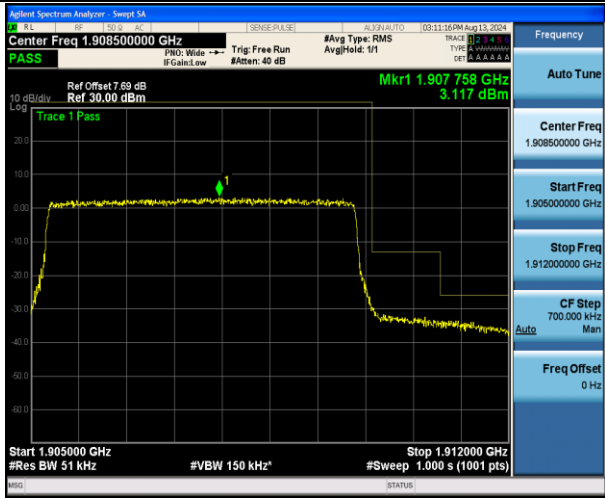
Band2_5MHz_16QAM_19175_25RB#0
