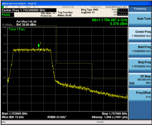
Band4_1.4MHz_16QAM_20393_6RB#0
