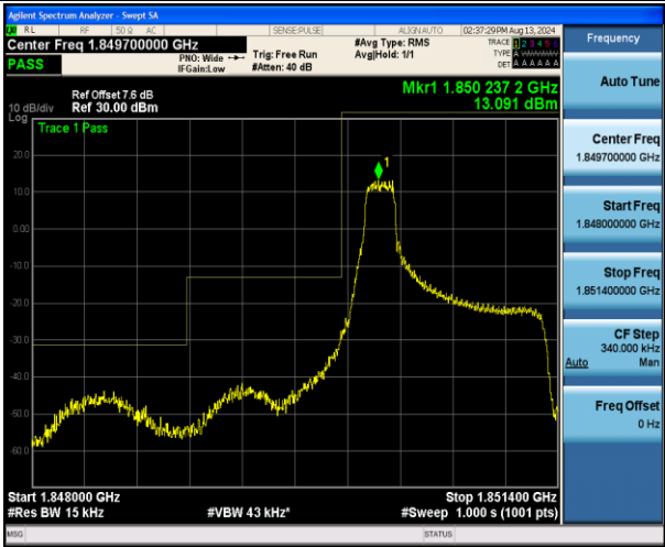
Band2_1.4MHz_16QAM_18607_1RB#0
