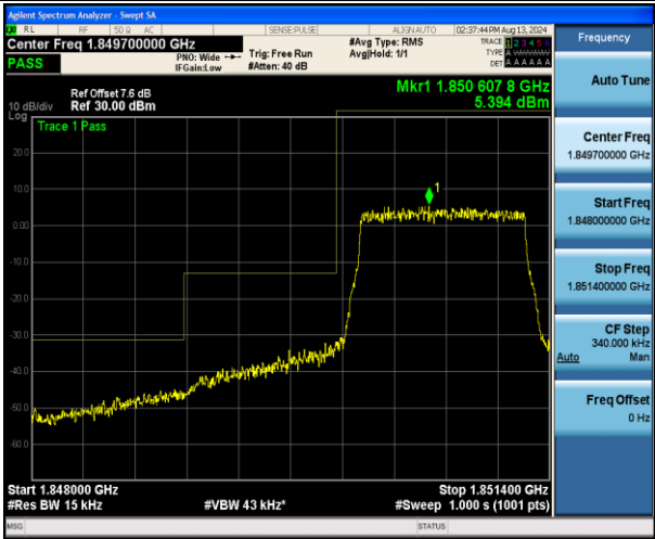
Band2_1.4MHz_16QAM_18607_6RB#0
